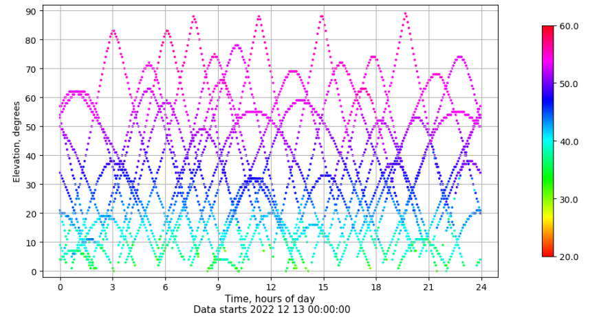
Time-elevation plot for station LPAL. Signal to Noise S1C Data file LPAL00ESP_R_2022347.xtr
