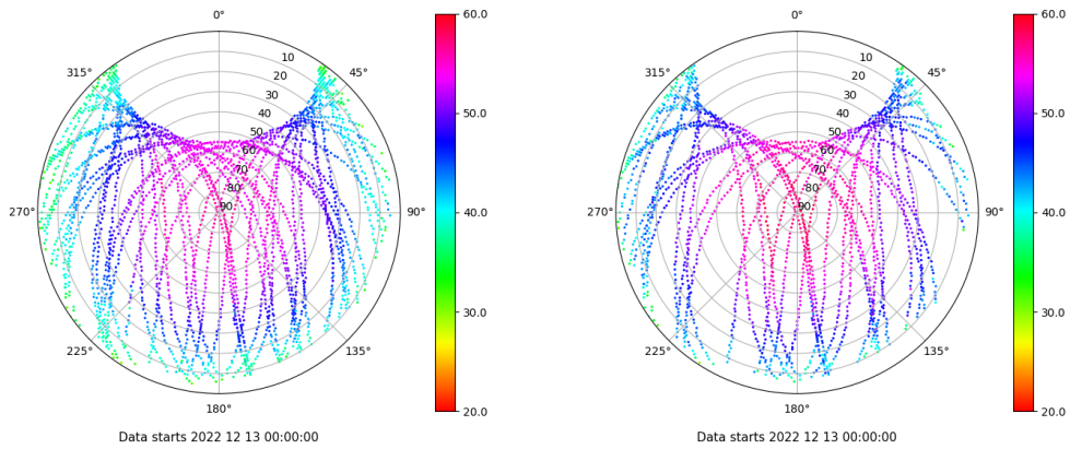
Skyplot for station LPAL. Signal to Noise S1C Data file LPAL00ESP_R_2022347.xtr Skyplot for station LPAL. Signal to Noise S2S Data file LPAL00ESP_R_2022347.xtr
