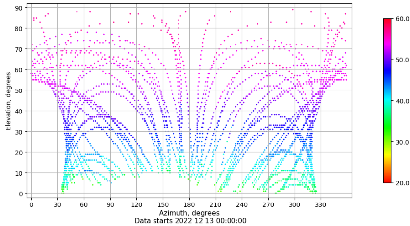
Azimuth-elevation plot for station LPAL. Signal to Noise S1C Data file LPAL00ESP_R_2022347.xtr
