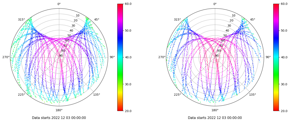
Skyplot for station LPAL. Signal to Noise S1C Data file LPAL00ESP_R_2022337.xtr Skyplot for station LPAL. Signal to Noise S2S Data file LPAL00ESP_R_2022337.xtr
