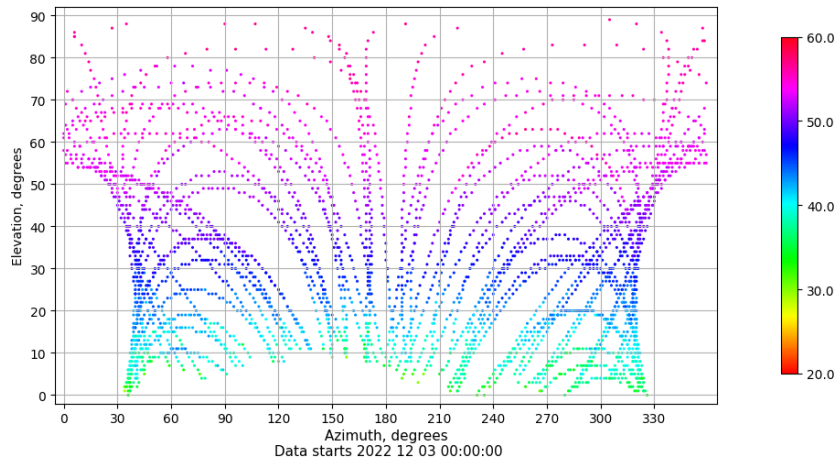
Azimuth-elevation plot for station LPAL. Signal to Noise S1C Data file LPAL00ESP_R_2022337.xtr
