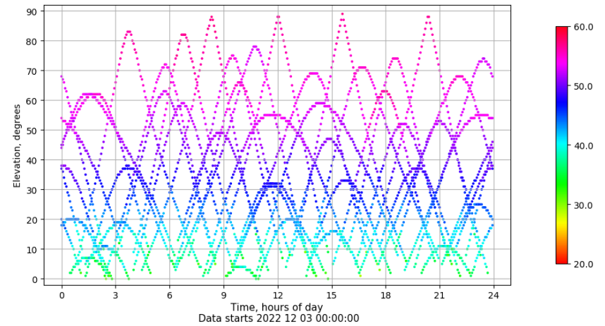
Time-elevation plot for station LPAL. Signal to Noise S1C Data file LPAL00ESP_R_2022337.xtr
