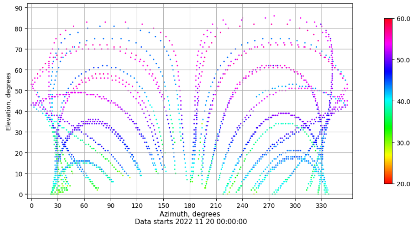
Azimuth-elevation plot for station LPAL. Signal to Noise S1C Data file LPAL00ESP_R_2022324.xtr
