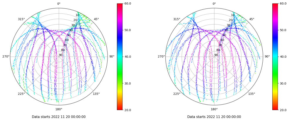
Skyplot for station LPAL. Signal to Noise S1C Data file LPAL00ESP_R_2022324.xtr Skyplot for station LPAL. Signal to Noise S2C Data file LPAL00ESP_R_2022324.xtr
