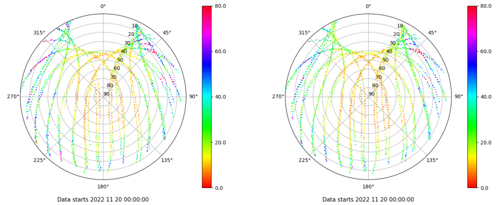
Skyplot for station LPAL. Parameter M1C Data file LPAL00ESP_R_2022324.xtr Skyplot for station LPAL. Parameter M2C Data file LPAL00ESP_R_2022324.xtr
