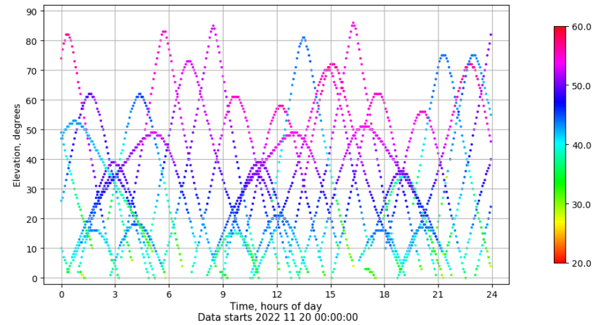
Time-elevation plot for station LPAL. Signal to Noise S1C Data file LPAL00ESP_R_2022324.xtr
