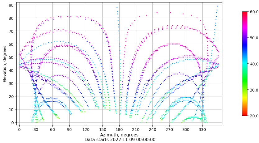
Azimuth-elevation plot for station LPAL. Signal to Noise S1C Data file LPAL00ESP_R_2022313.xtr
