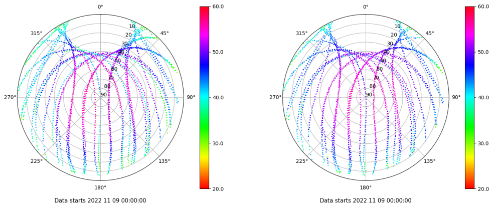
Skyplot for station LPAL. Signal to Noise S1C Data file LPAL00ESP_R_2022313.xtr Skyplot for station LPAL. Signal to Noise S2C Data file LPAL00ESP_R_2022313.xtr
