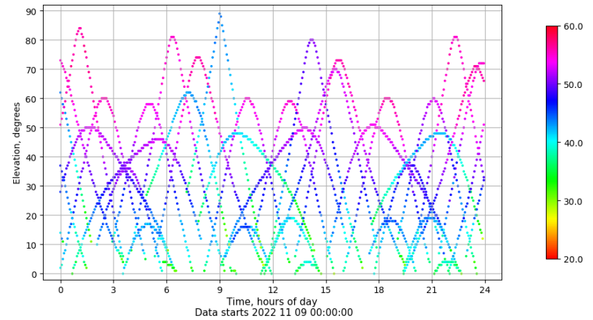
Time-elevation plot for station LPAL. Signal to Noise S1C Data file LPAL00ESP_R_2022313.xtr
