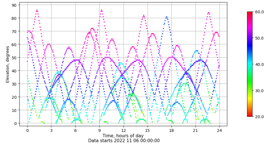
Time-elevation plot for station LPAL. Signal to Noise S1C Data file LPAL00ESP_R_2022310.xtr
