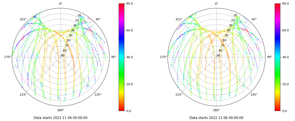
Skyplot for station LPAL. Parameter M1C Data file LPAL00ESP_R_2022310.xtr Skyplot for station LPAL. Parameter M2C Data file LPAL00ESP_R_2022310.xtr
