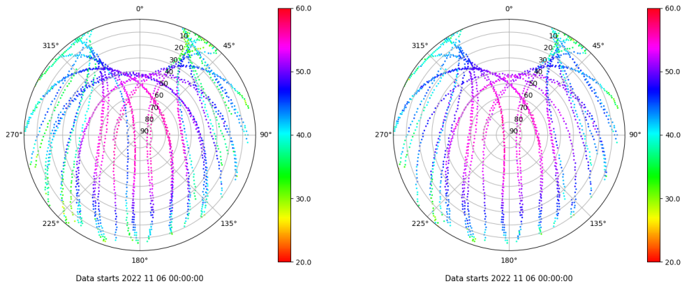
Skyplot for station LPAL. Signal to Noise S1C Data file LPAL00ESP_R_2022310.xtr Skyplot for station LPAL. Signal to Noise S2C Data file LPAL00ESP_R_2022310.xtr
