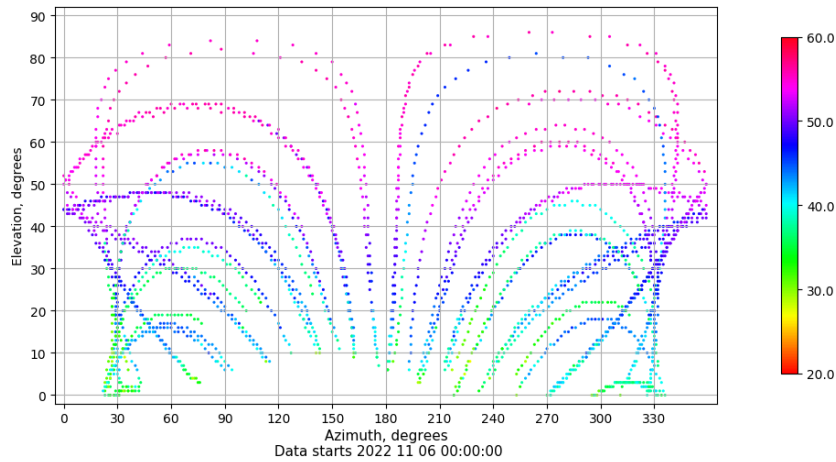
Azimuth-elevation plot for station LPAL. Signal to Noise S1C Data file LPAL00ESP_R_2022310.xtr
