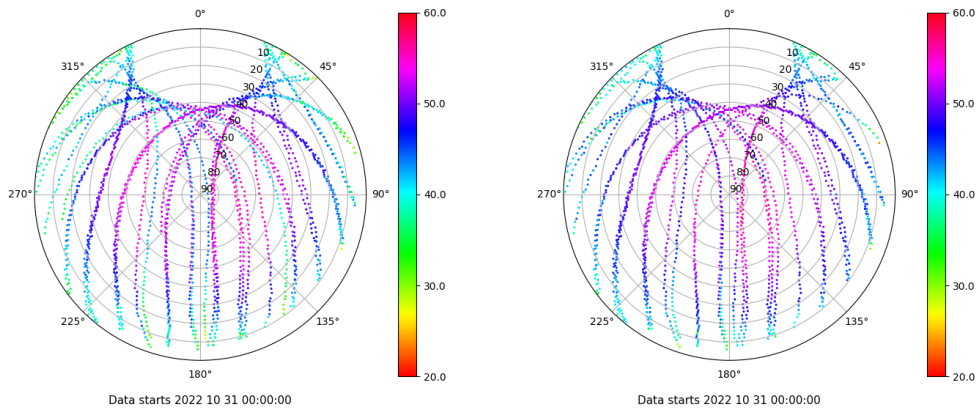
Skyplot for station LPAL. Signal to Noise S1C Data file LPAL00ESP_R_2022304.xtr Skyplot for station LPAL. Signal to Noise S2C Data file LPAL00ESP_R_2022304.xtr
