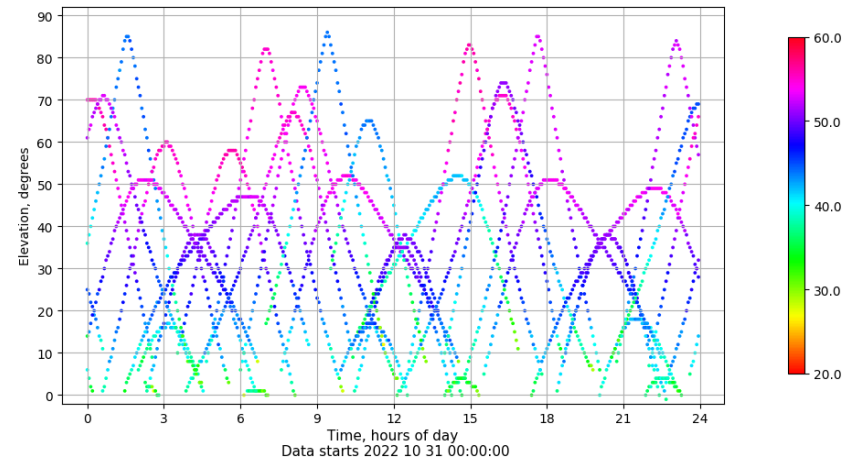
Time-elevation plot for station LPAL. Signal to Noise S1C Data file LPAL00ESP_R_2022304.xtr
