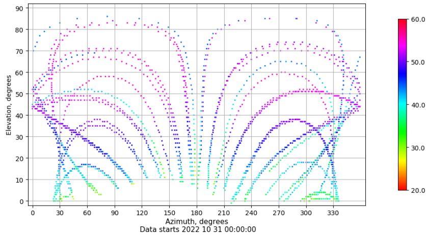
Azimuth-elevation plot for station LPAL. Signal to Noise S1C Data file LPAL00ESP_R_2022304.xtr
