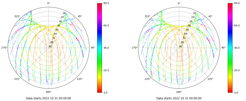
Skyplot for station LPAL. Parameter M1C Data file LPAL00ESP_R_2022304.xtr Skyplot for station LPAL. Parameter M2C Data file LPAL00ESP_R_2022304.xtr
