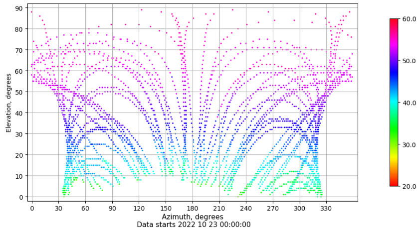
Azimuth-elevation plot for station LPAL. Signal to Noise S1C Data file LPAL00ESP_R_2022296.xtr
