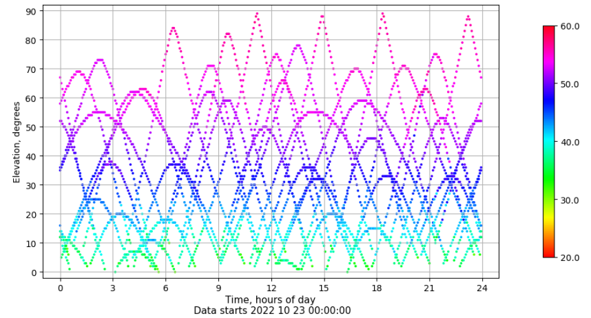
Time-elevation plot for station LPAL. Signal to Noise S1C Data file LPAL00ESP_R_2022296.xtr
