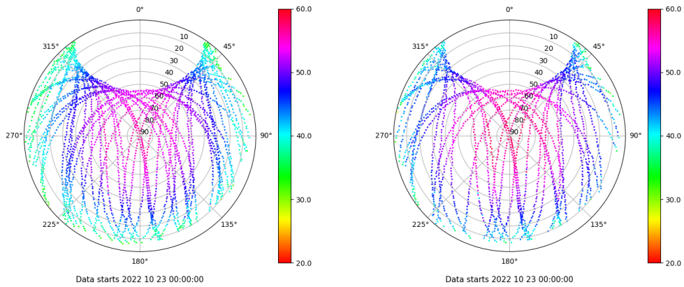
Skyplot for station LPAL. Signal to Noise S1C Data file LPAL00ESP_R_2022296.xtr Skyplot for station LPAL. Signal to Noise S2S Data file LPAL00ESP_R_2022296.xtr
