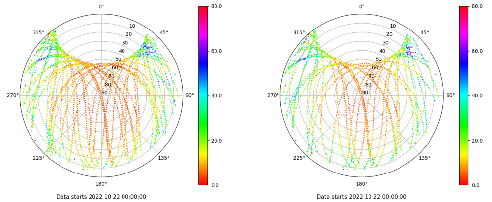
Skyplot for station LPAL. Parameter M1C Data file LPAL00ESP_R_2022295.xtr Skyplot for station LPAL. Parameter M2S Data file LPAL00ESP_R_2022295.xtr
