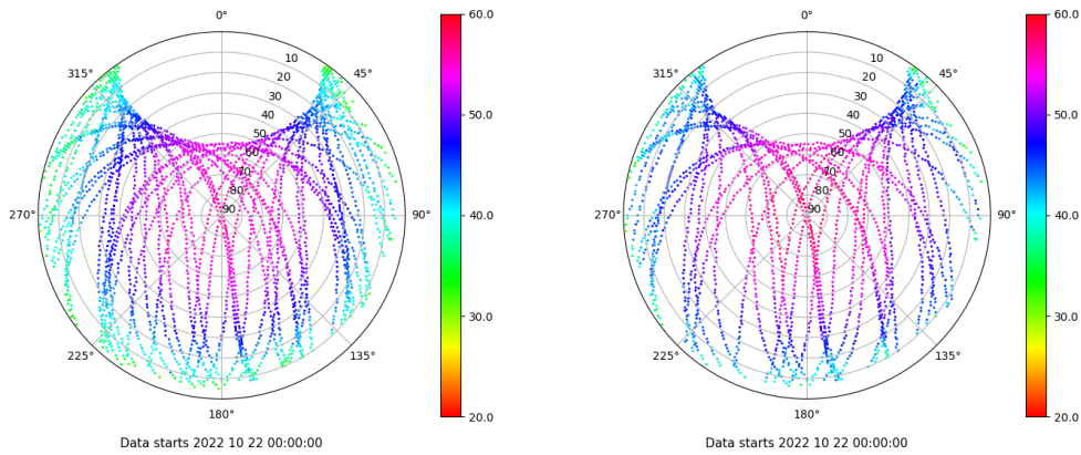
Skyplot for station LPAL. Signal to Noise S1C Data file LPAL00ESP_R_2022295.xtr Skyplot for station LPAL. Signal to Noise S2S Data file LPAL00ESP_R_2022295.xtr
