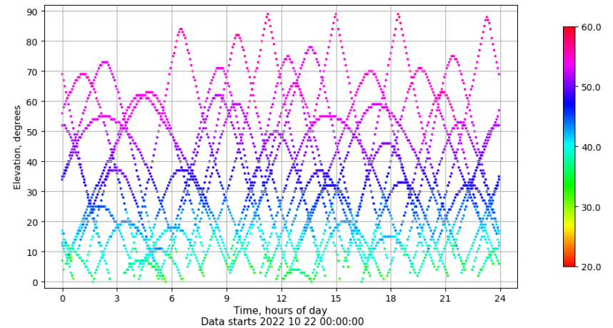
Time-elevation plot for station LPAL. Signal to Noise S1C Data file LPAL00ESP_R_2022295.xtr
