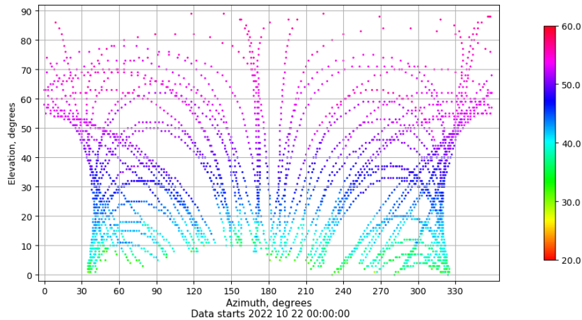
Azimuth-elevation plot for station LPAL. Signal to Noise S1C Data file LPAL00ESP_R_2022295.xtr
