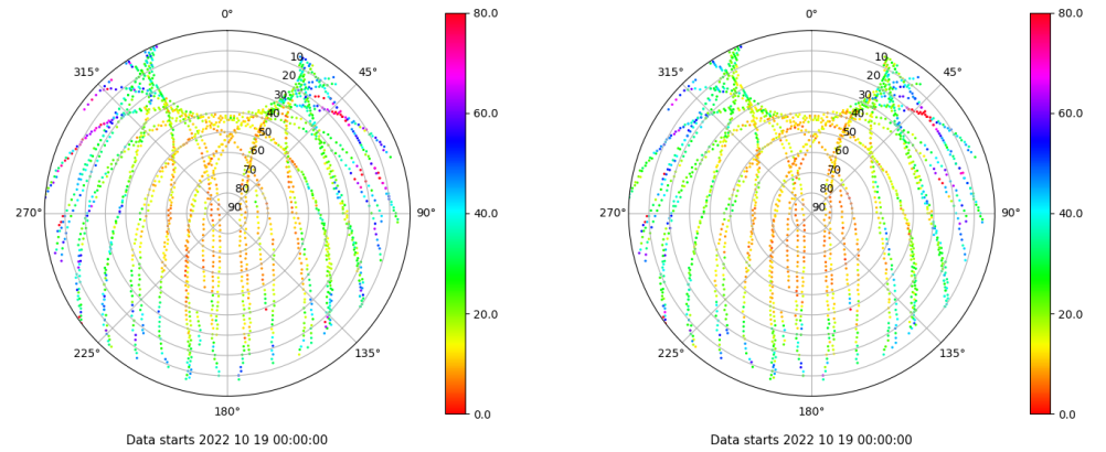
Skyplot for station LPAL. Parameter M1C Data file LPAL00ESP_R_2022292.xtr Skyplot for station LPAL. Parameter M2C Data file LPAL00ESP_R_2022292.xtr
