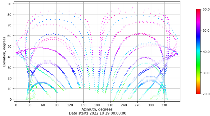
Azimuth-elevation plot for station LPAL. Signal to Noise S1C Data file LPAL00ESP_R_2022292.xtr
