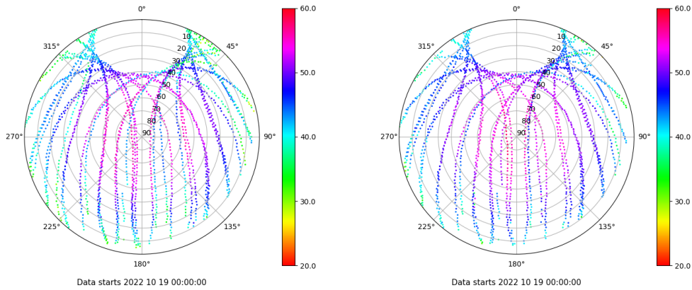
Skyplot for station LPAL. Signal to Noise S1C Data file LPAL00ESP_R_2022292.xtr Skyplot for station LPAL. Signal to Noise S2C Data file LPAL00ESP_R_2022292.xtr
