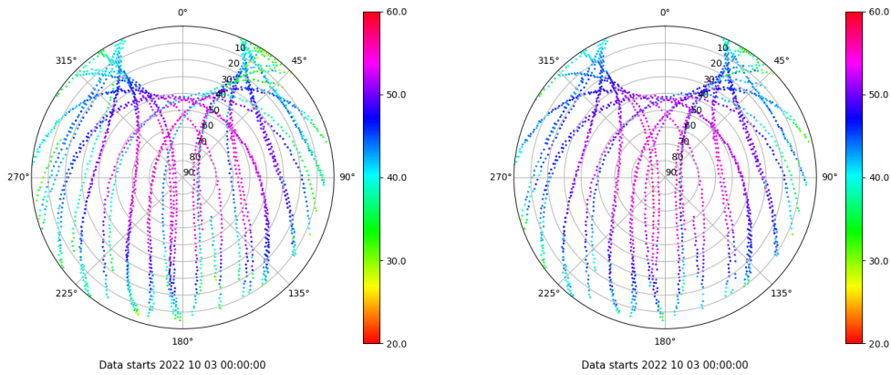
Skyplot for station LPAL. Signal to Noise S1C Data file LPAL00ESP_R_2022276.xtr Skyplot for station LPAL. Signal to Noise S2C Data file LPAL00ESP_R_2022276.xtr
