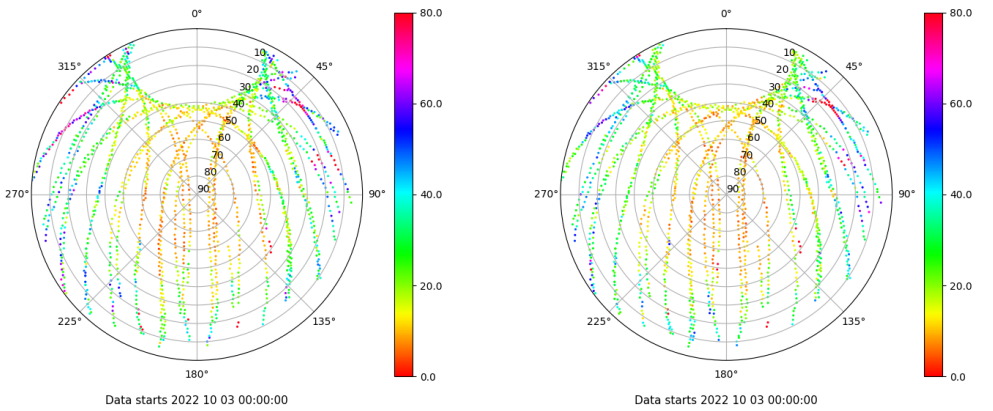
Skyplot for station LPAL. Parameter M1C Data file LPAL00ESP_R_2022276.xtr Skyplot for station LPAL. Parameter M2C Data file LPAL00ESP_R_2022276.xtr
