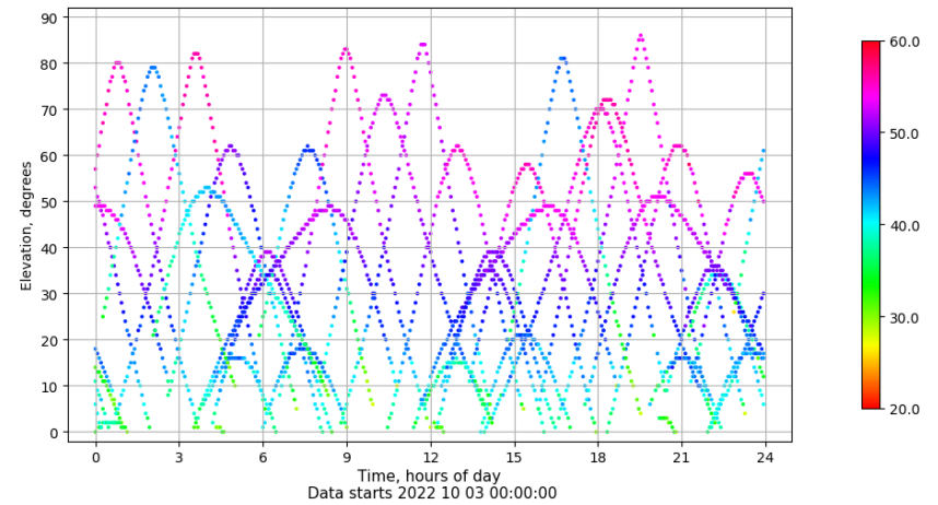
Time-elevation plot for station LPAL. Signal to Noise S1C Data file LPAL00ESP_R_2022276.xtr
