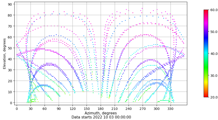
Azimuth-elevation plot for station LPAL. Signal to Noise S1C Data file LPAL00ESP_R_2022276.xtr
