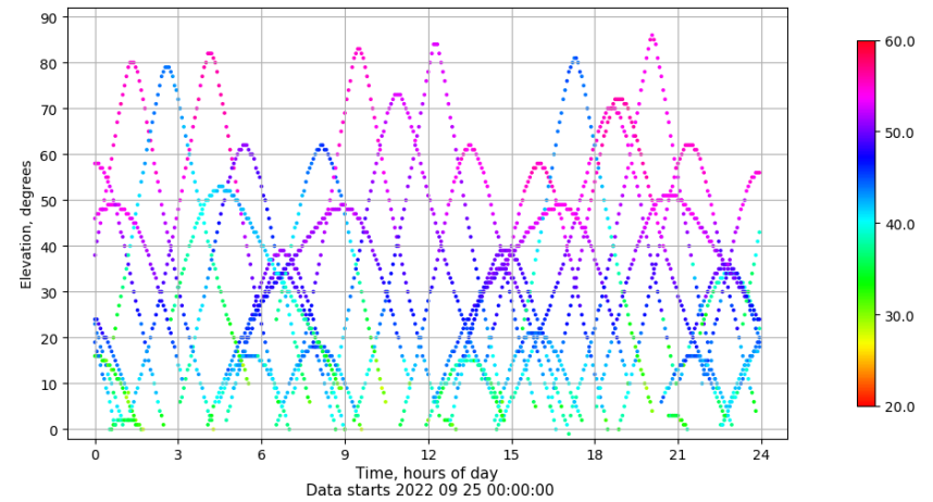
Time-elevation plot for station LPAL. Signal to Noise S1C Data file LPAL00ESP_R_2022268.xtr
