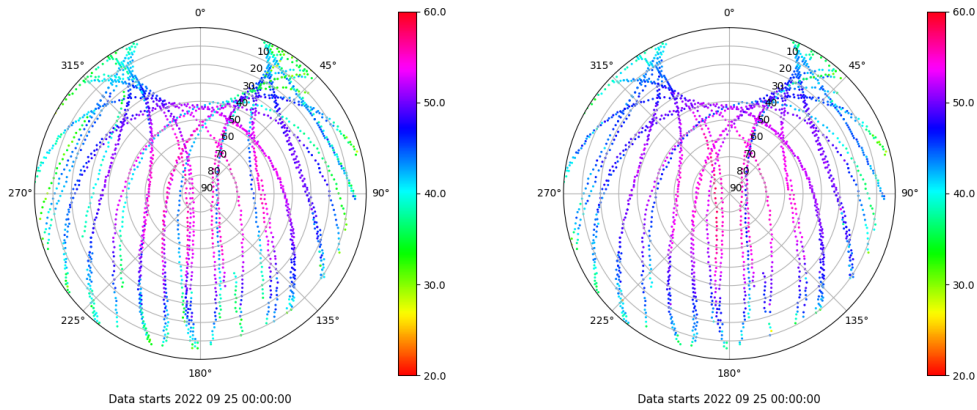
Skyplot for station LPAL. Signal to Noise S1C Data file LPAL00ESP_R_2022268.xtr Skyplot for station LPAL. Signal to Noise S2C Data file LPAL00ESP_R_2022268.xtr
