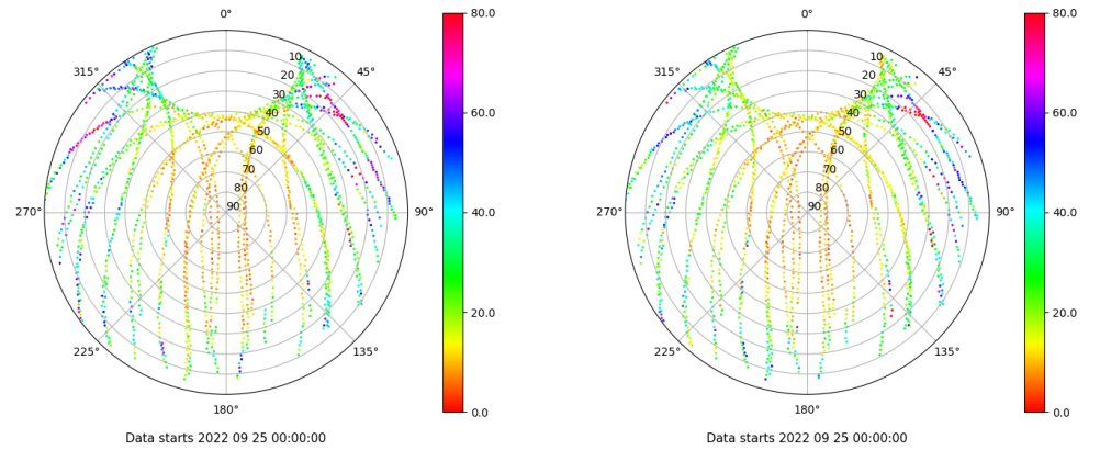
Skyplot for station LPAL. Parameter M1C Data file LPAL00ESP_R_2022268.xtr Skyplot for station LPAL. Parameter M2C Data file LPAL00ESP_R_2022268.xtr
