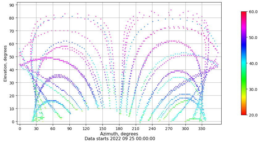
Azimuth-elevation plot for station LPAL. Signal to Noise S1C Data file LPAL00ESP_R_2022268.xtr
