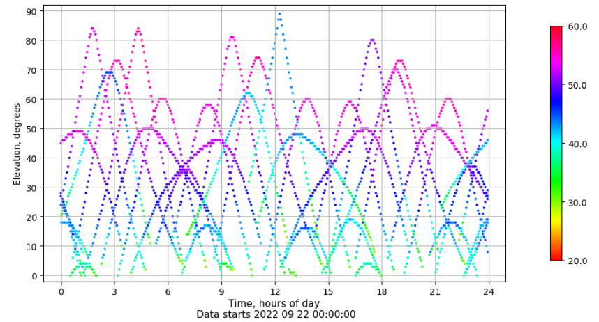
Time-elevation plot for station LPAL. Signal to Noise S1C Data file LPAL00ESP_R_2022265.xtr
