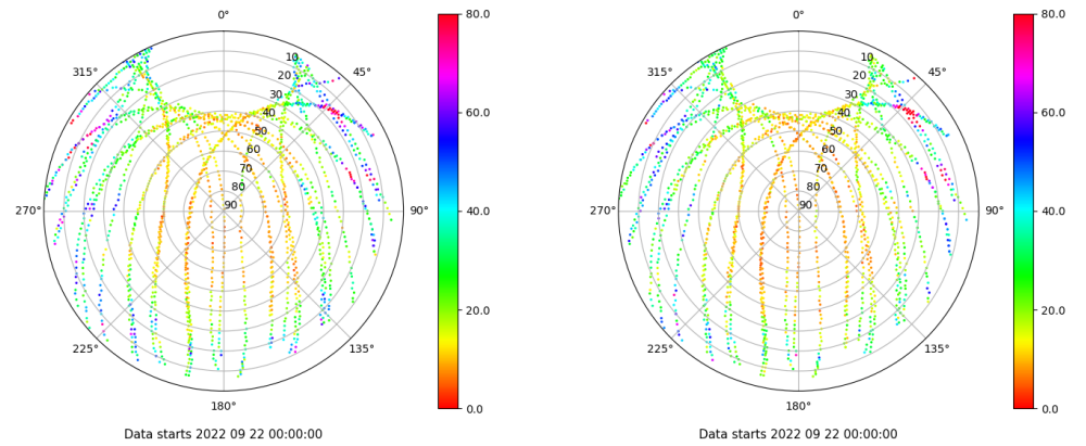
Skyplot for station LPAL. Parameter M1C Data file LPAL00ESP_R_2022265.xtr Skyplot for station LPAL. Parameter M2C Data file LPAL00ESP_R_2022265.xtr
