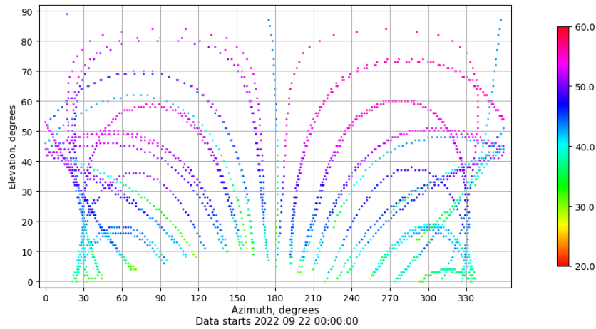
Azimuth-elevation plot for station LPAL. Signal to Noise S1C Data file LPAL00ESP_R_2022265.xtr
