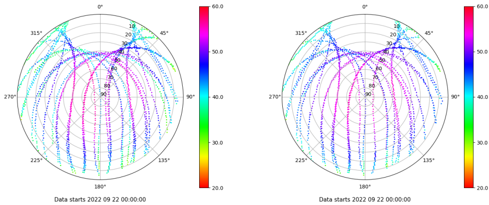
Skyplot for station LPAL. Signal to Noise S1C Data file LPAL00ESP_R_2022265.xtr Skyplot for station LPAL. Signal to Noise S2C Data file LPAL00ESP_R_2022265.xtr
