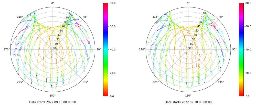
Skyplot for station LPAL. Parameter M1C Data file LPAL00ESP_R_2022261.xtr Skyplot for station LPAL. Parameter M2C Data file LPAL00ESP_R_2022261.xtr
