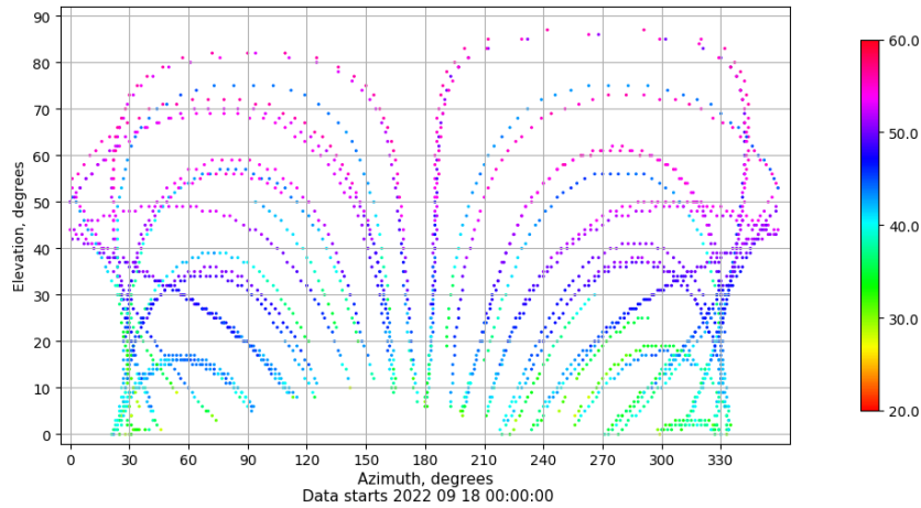
Azimuth-elevation plot for station LPAL. Signal to Noise S1C Data file LPAL00ESP_R_2022261.xtr
