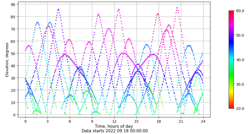
Time-elevation plot for station LPAL. Signal to Noise S1C Data file LPAL00ESP_R_2022261.xtr
