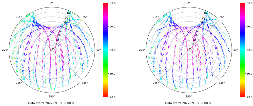
Skyplot for station LPAL. Signal to Noise S1C Data file LPAL00ESP_R_2022261.xtr Skyplot for station LPAL. Signal to Noise S2C Data file LPAL00ESP_R_2022261.xtr
