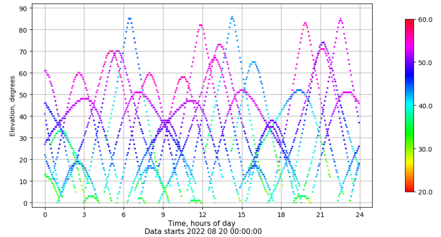
Time-elevation plot for station LPAL. Signal to Noise S1C Data file LPAL00ESP_R_2022232.xtr
