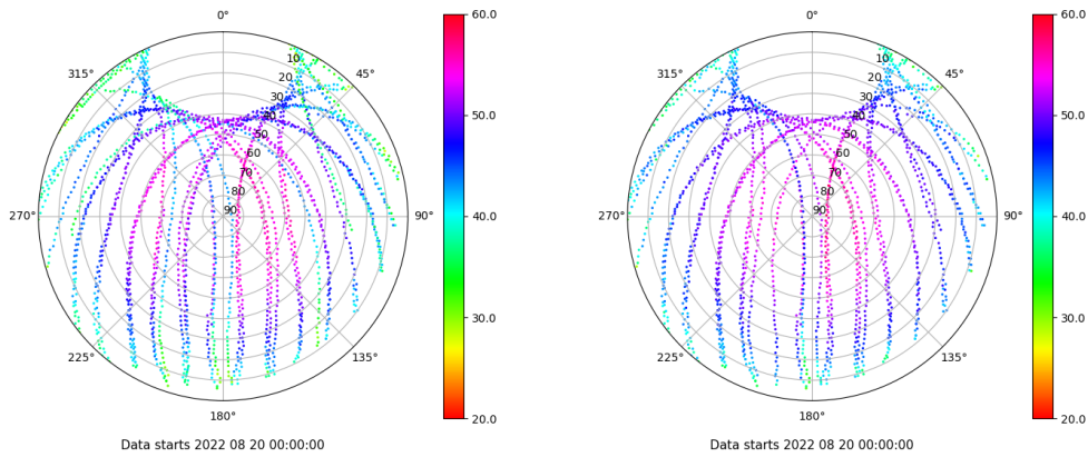
Skyplot for station LPAL. Signal to Noise S1C Data file LPAL00ESP_R_2022232.xtr Skyplot for station LPAL. Signal to Noise S2C Data file LPAL00ESP_R_2022232.xtr
