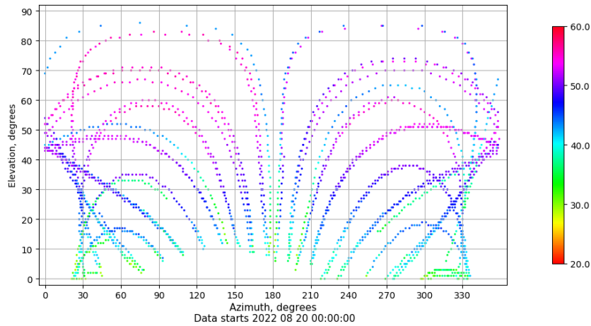
Azimuth-elevation plot for station LPAL. Signal to Noise S1C Data file LPAL00ESP_R_2022232.xtr
