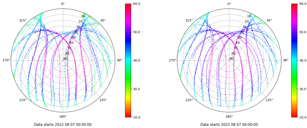
Skyplot for station LPAL. Signal to Noise S1C Data file LPAL00ESP_R_2022219.xtr Skyplot for station LPAL. Signal to Noise S2C Data file LPAL00ESP_R_2022219.xtr
