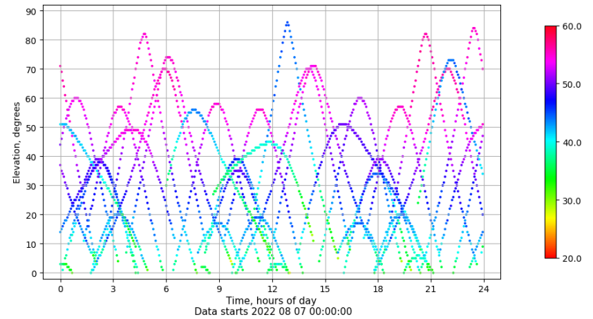
Time-elevation plot for station LPAL. Signal to Noise S1C Data file LPAL00ESP_R_2022219.xtr
