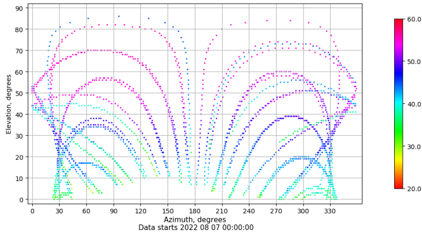
Azimuth-elevation plot for station LPAL. Signal to Noise S1C Data file LPAL00ESP_R_2022219.xtr
