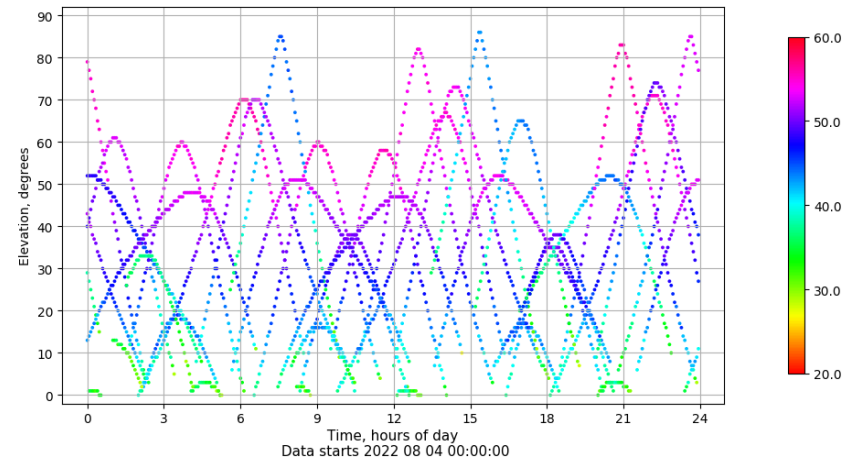
Time-elevation plot for station LPAL. Signal to Noise S1C Data file LPAL00ESP_R_2022216.xtr
