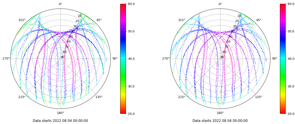
Skyplot for station LPAL. Signal to Noise S1C Data file LPAL00ESP_R_2022216.xtr Skyplot for station LPAL. Signal to Noise S2C Data file LPAL00ESP_R_2022216.xtr
