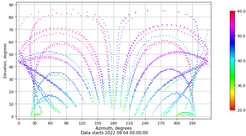
Azimuth-elevation plot for station LPAL. Signal to Noise S1C Data file LPAL00ESP_R_2022216.xtr
