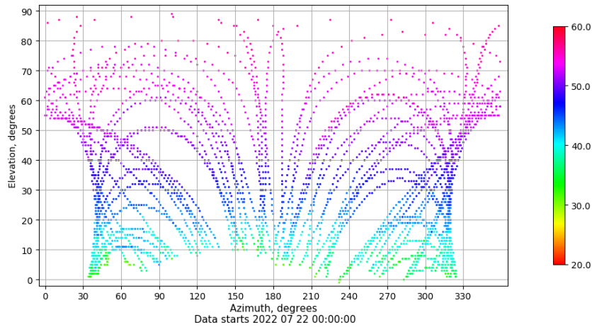
Azimuth-elevation plot for station LPAL. Signal to Noise S1C Data file LPAL00ESP_R_2022203.xtr
