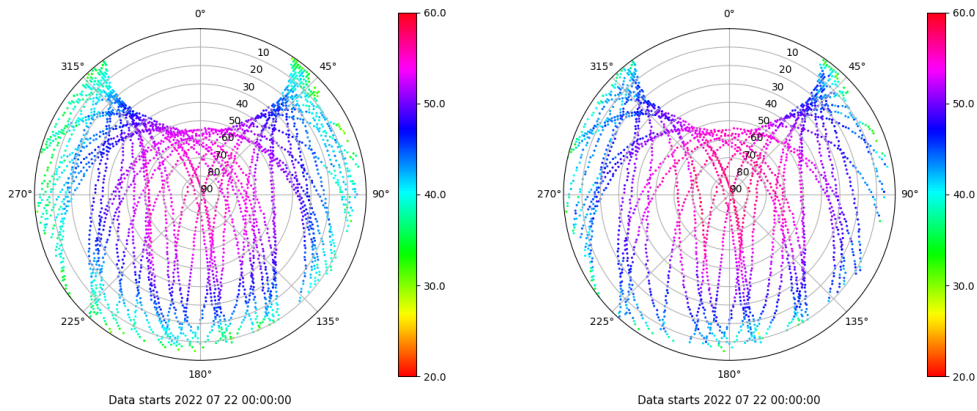
Skyplot for station LPAL. Signal to Noise S1C Data file LPAL00ESP_R_2022203.xtr Skyplot for station LPAL. Signal to Noise S2S Data file LPAL00ESP_R_2022203.xtr
