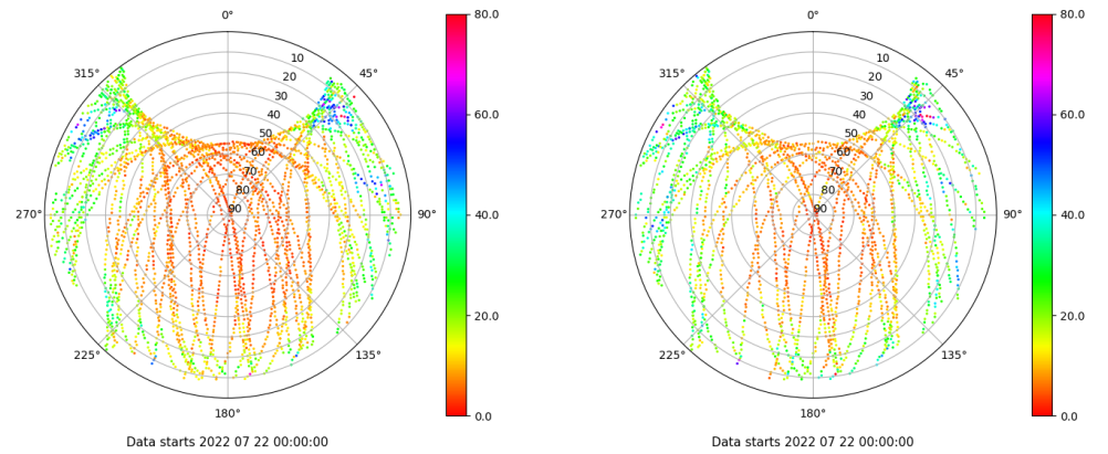
Skyplot for station LPAL. Parameter M1C Data file LPAL00ESP_R_2022203.xtr Skyplot for station LPAL. Parameter M2S Data file LPAL00ESP_R_2022203.xtr
