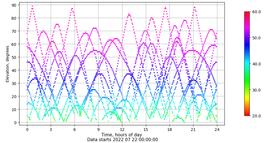
Time-elevation plot for station LPAL. Signal to Noise S1C Data file LPAL00ESP_R_2022203.xtr
