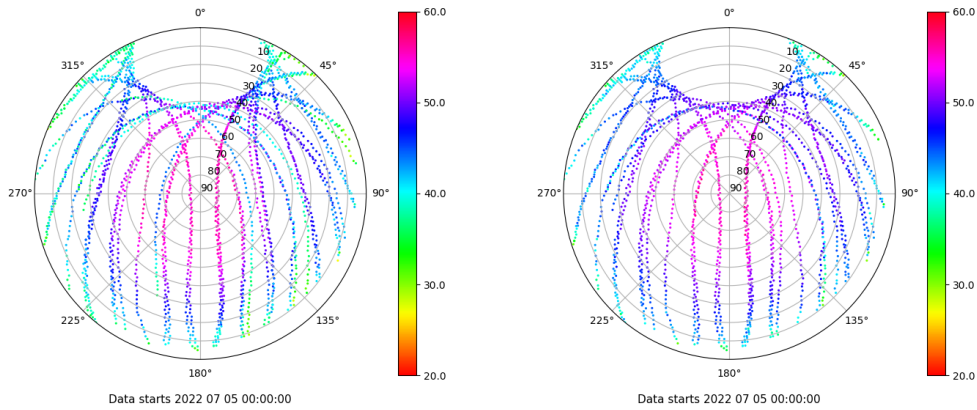
Skyplot for station LPAL. Signal to Noise S1C Data file LPAL00ESP_R_2022186.xtr Skyplot for station LPAL. Signal to Noise S2C Data file LPAL00ESP_R_2022186.xtr
