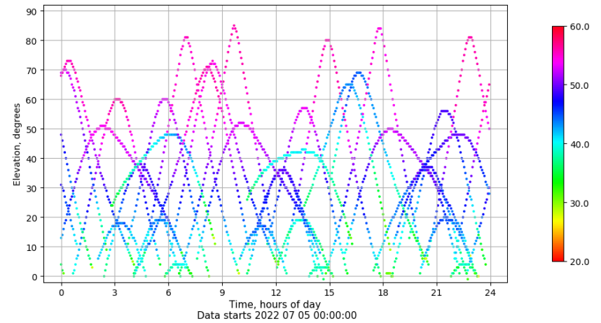
Time-elevation plot for station LPAL. Signal to Noise S1C Data file LPAL00ESP_R_2022186.xtr
