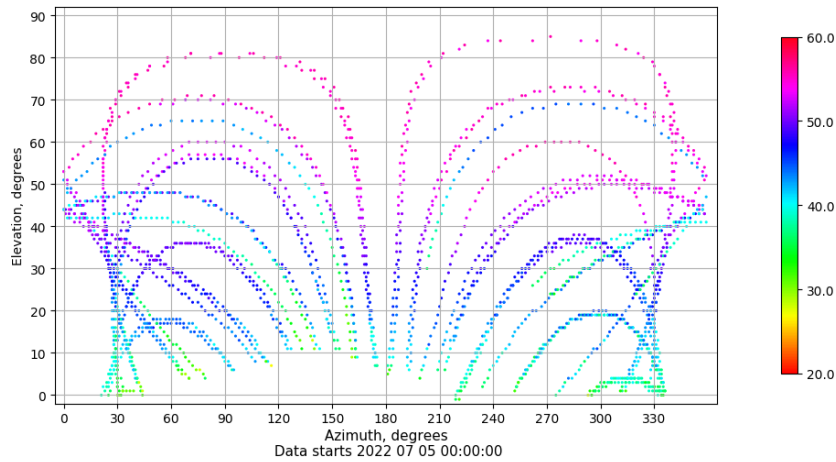
Azimuth-elevation plot for station LPAL. Signal to Noise S1C Data file LPAL00ESP_R_2022186.xtr
