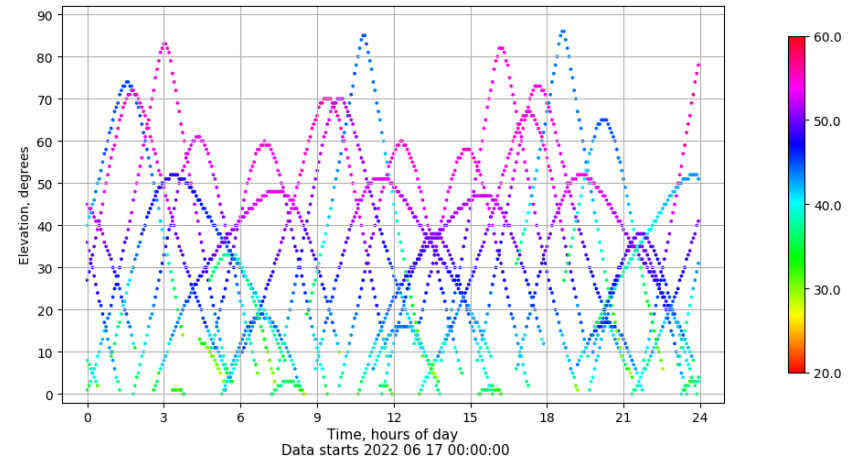
Time-elevation plot for station LPAL. Signal to Noise S1C Data file LPAL00ESP_R_2022168.xtr
