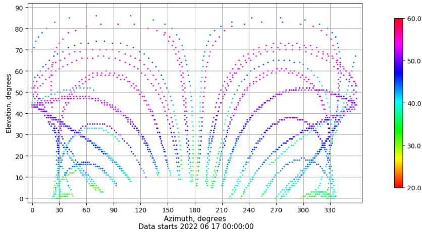
Azimuth-elevation plot for station LPAL. Signal to Noise S1C Data file LPAL00ESP_R_2022168.xtr
