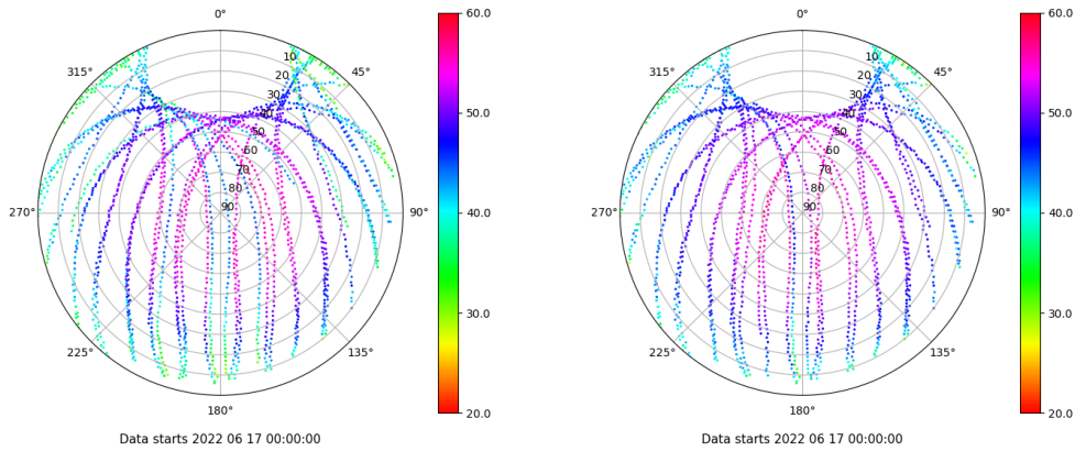
Skyplot for station LPAL. Signal to Noise S1C Data file LPAL00ESP_R_2022168.xtr Skyplot for station LPAL. Signal to Noise S2C Data file LPAL00ESP_R_2022168.xtr
