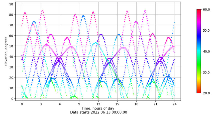
Time-elevation plot for station LPAL. Signal to Noise S1C Data file LPAL00ESP_R_2022164.xtr
