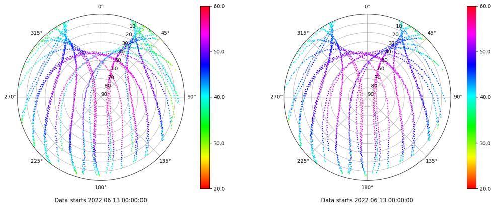
Skyplot for station LPAL. Signal to Noise S1C Data file LPAL00ESP_R_2022164.xtr Skyplot for station LPAL. Signal to Noise S2C Data file LPAL00ESP_R_2022164.xtr
