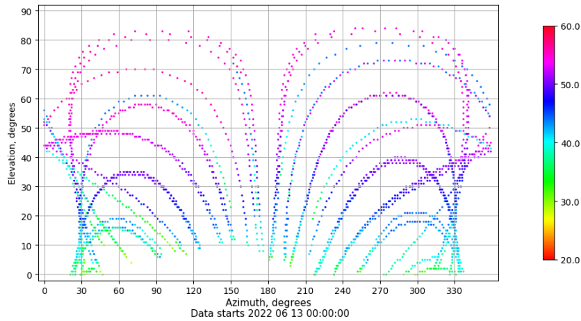
Azimuth-elevation plot for station LPAL. Signal to Noise S1C Data file LPAL00ESP_R_2022164.xtr
