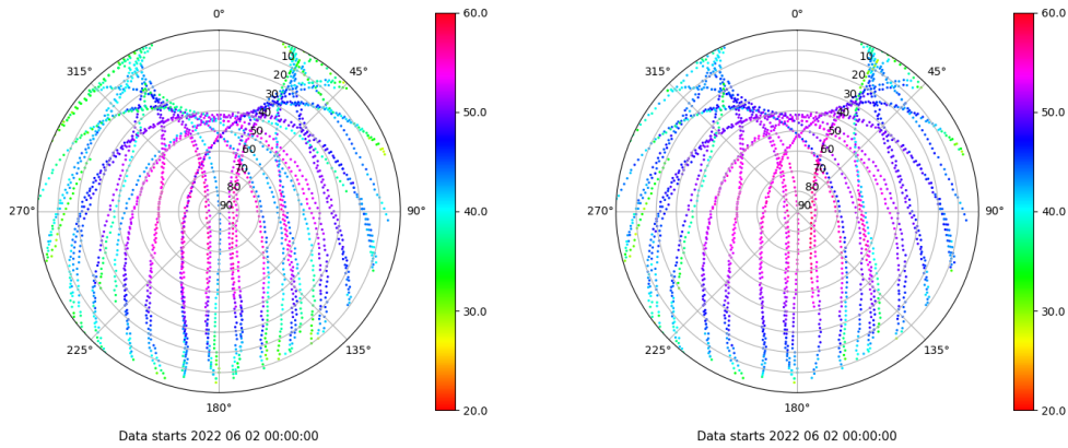
Skyplot for station LPAL. Signal to Noise S1C Data file LPAL00ESP_R_2022153.xtr Skyplot for station LPAL. Signal to Noise S2C Data file LPAL00ESP_R_2022153.xtr
