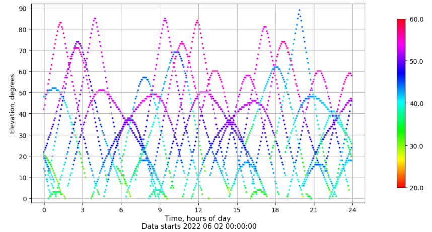
Time-elevation plot for station LPAL. Signal to Noise S1C Data file LPAL00ESP_R_2022153.xtr
