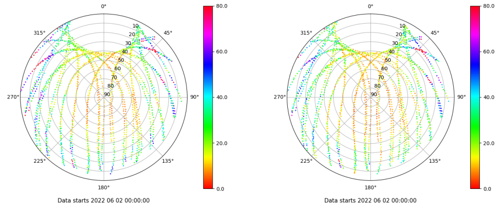
Skyplot for station LPAL. Parameter M1C Data file LPAL00ESP_R_2022153.xtr Skyplot for station LPAL. Parameter M2C Data file LPAL00ESP_R_2022153.xtr
