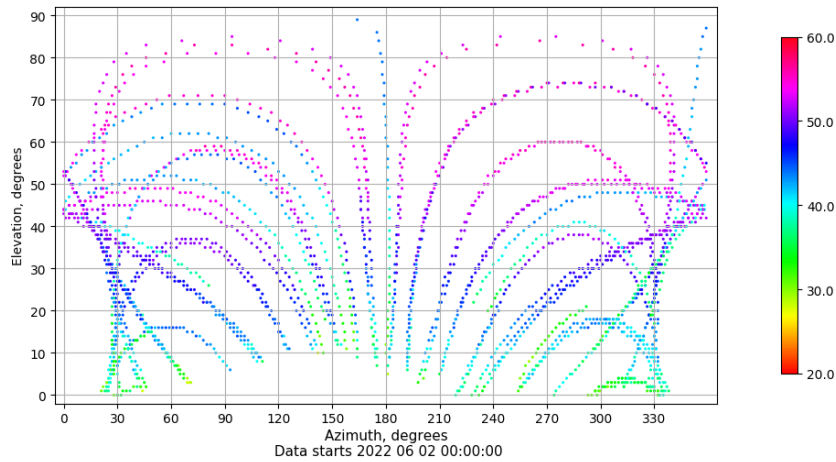
Azimuth-elevation plot for station LPAL. Signal to Noise S1C Data file LPAL00ESP_R_2022153.xtr
