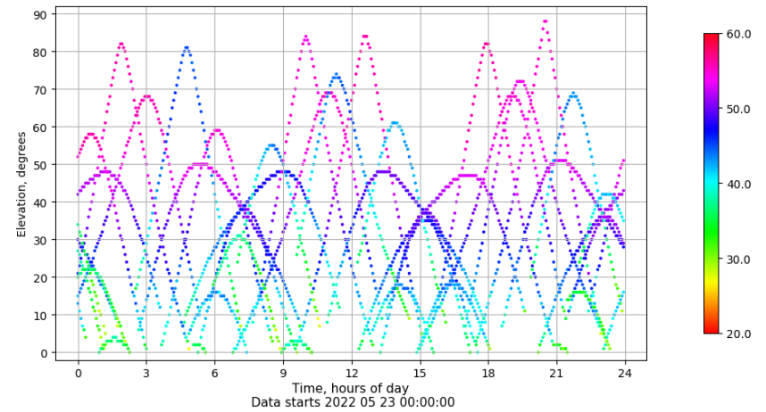
Time-elevation plot for station LPAL. Signal to Noise S1C Data file LPAL00ESP_R_2022143.xtr
