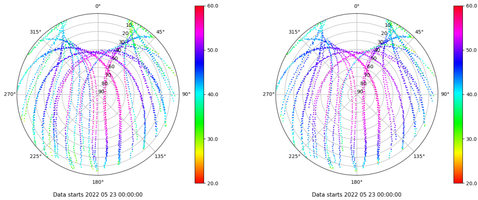
Skyplot for station LPAL. Signal to Noise S1C Data file LPAL00ESP_R_2022143.xtr Skyplot for station LPAL. Signal to Noise S2C Data file LPAL00ESP_R_2022143.xtr
