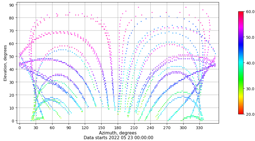
Azimuth-elevation plot for station LPAL. Signal to Noise S1C Data file LPAL00ESP_R_2022143.xtr
