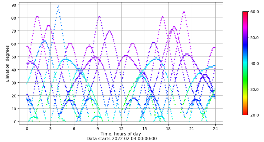
Time-elevation plot for station LPAL. Signal to Noise S1C Data file LPAL00ESP_R_2022034.xtr
