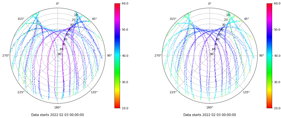
Skyplot for station LPAL. Signal to Noise S1C Data file LPAL00ESP_R_2022034.xtr Skyplot for station LPAL. Signal to Noise S2P Data file LPAL00ESP_R_2022034.xtr
