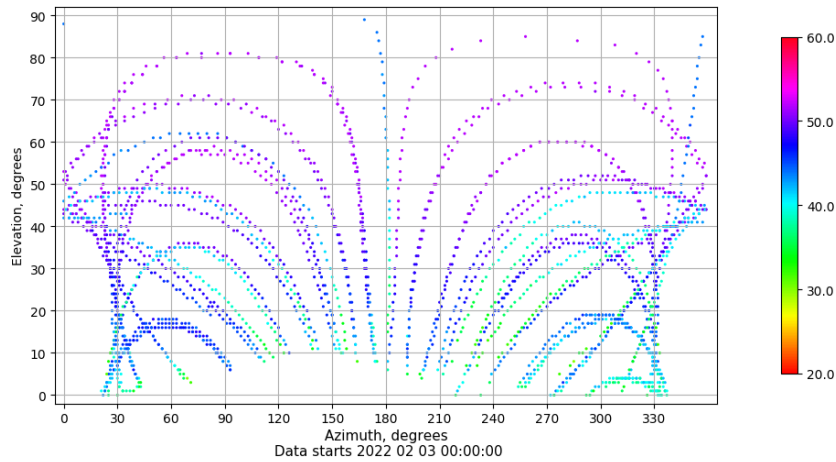
Azimuth-elevation plot for station LPAL. Signal to Noise S1C Data file LPAL00ESP_R_2022034.xtr
