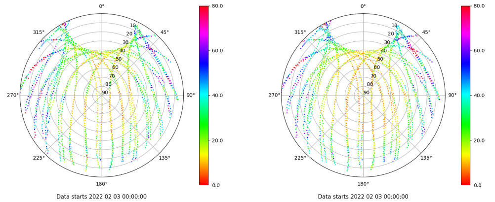
Skyplot for station LPAL. Parameter M1C Data file LPAL00ESP_R_2022034.xtr Skyplot for station LPAL. Parameter M2P Data file LPAL00ESP_R_2022034.xtr
