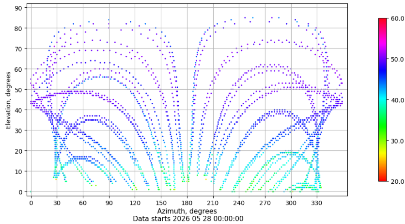
Azimuth-elevation plot for station LP01. Signal to Noise S1C Data file LP0100ESP_R_2026148.xtr
