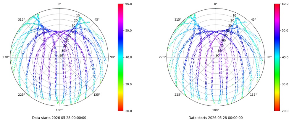
Skyplot for station LP01. Signal to Noise S1C Data file LP0100ESP_R_2026148.xtr Skyplot for station LP01. Signal to Noise S2C Data file LP0100ESP_R_2026148.xtr
