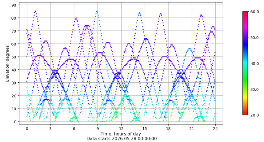
Time-elevation plot for station LP01. Signal to Noise S1C Data file LP0100ESP_R_2026148.xtr
