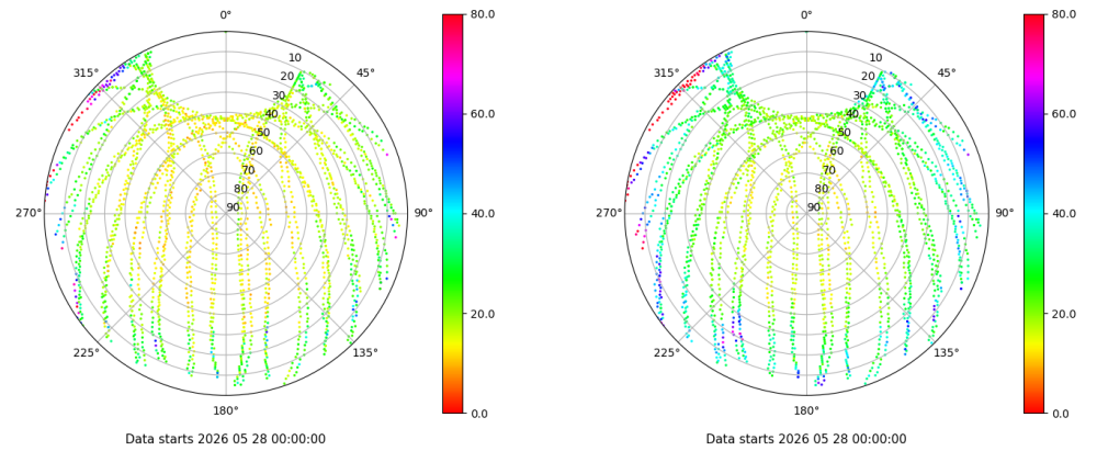
Skyplot for station LP01. Parameter M1C Data file LP0100ESP_R_2026148.xtr Skyplot for station LP01. Parameter M2C Data file LP0100ESP_R_2026148.xtr
