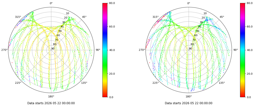
Skyplot for station LP01. Parameter M1C Data file LP0100ESP_R_2026142.xtr Skyplot for station LP01. Parameter M2C Data file LP0100ESP_R_2026142.xtr
