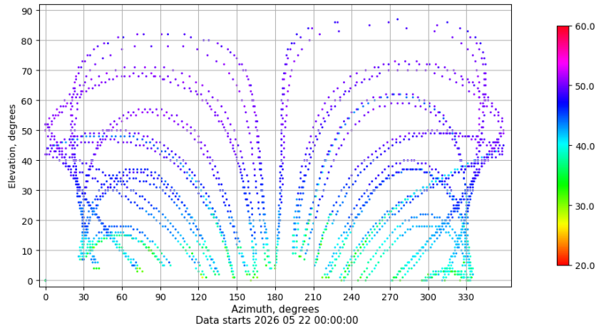
Azimuth-elevation plot for station LP01. Signal to Noise S1C Data file LP0100ESP_R_2026142.xtr
