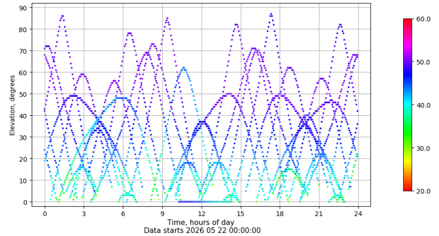
Time-elevation plot for station LP01. Signal to Noise S1C Data file LP0100ESP_R_2026142.xtr
