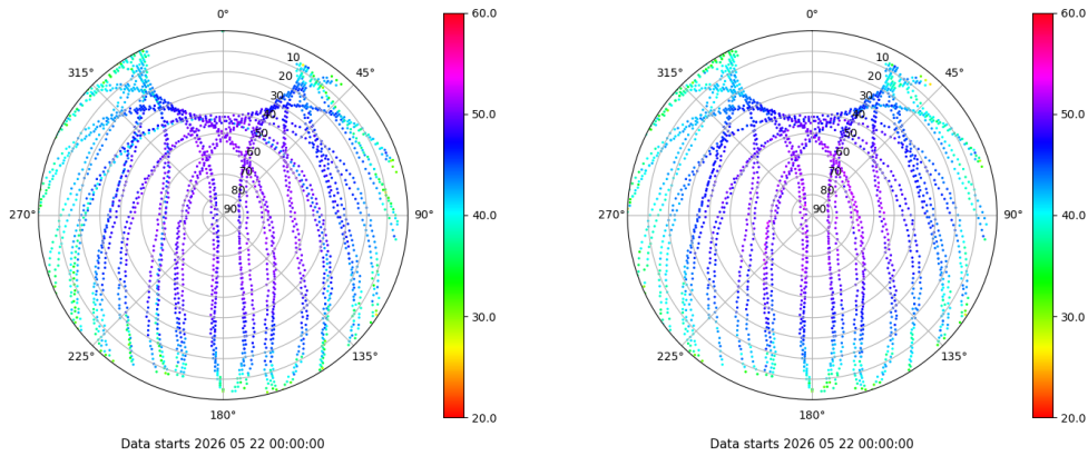
Skyplot for station LP01. Signal to Noise S1C Data file LP0100ESP_R_2026142.xtr Skyplot for station LP01. Signal to Noise S2C Data file LP0100ESP_R_2026142.xtr
