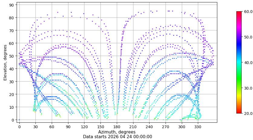
Azimuth-elevation plot for station LP01. Signal to Noise S1C Data file LP0100ESP_R_2026114.xtr
