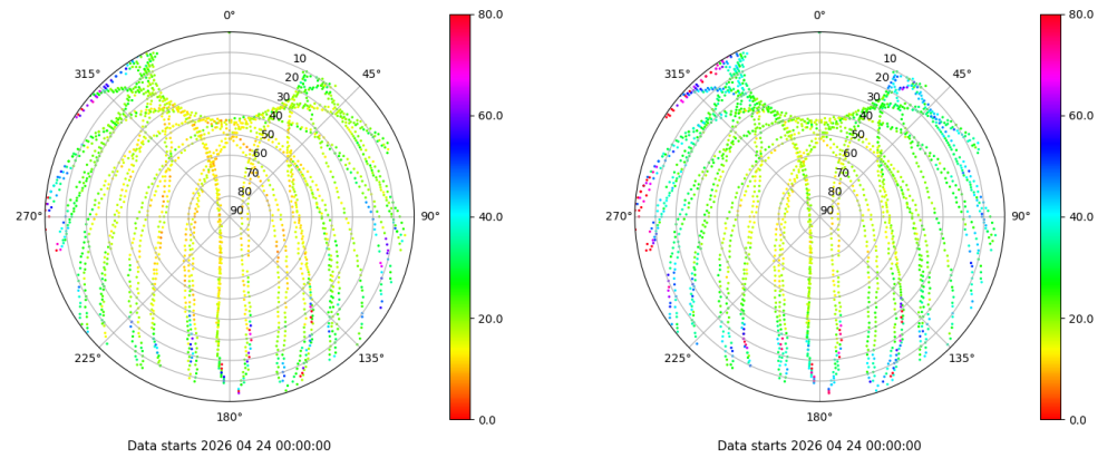
Skyplot for station LP01. Parameter M1C Data file LP0100ESP_R_2026114.xtr Skyplot for station LP01. Parameter M2C Data file LP0100ESP_R_2026114.xtr
