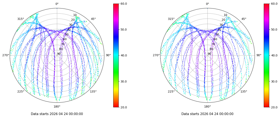
Skyplot for station LP01. Signal to Noise S1C Data file LP0100ESP_R_2026114.xtr Skyplot for station LP01. Signal to Noise S2C Data file LP0100ESP_R_2026114.xtr
