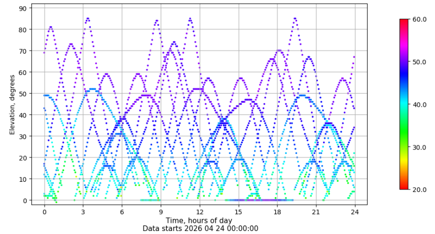
Time-elevation plot for station LP01. Signal to Noise S1C Data file LP0100ESP_R_2026114.xtr
