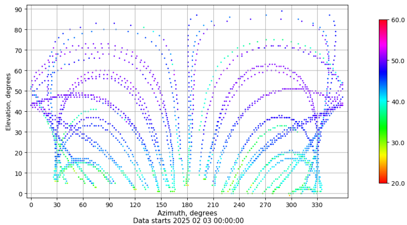
Azimuth-elevation plot for station LP01. Signal to Noise S1C Data file LP0100ESP_R_2025034.xtr
