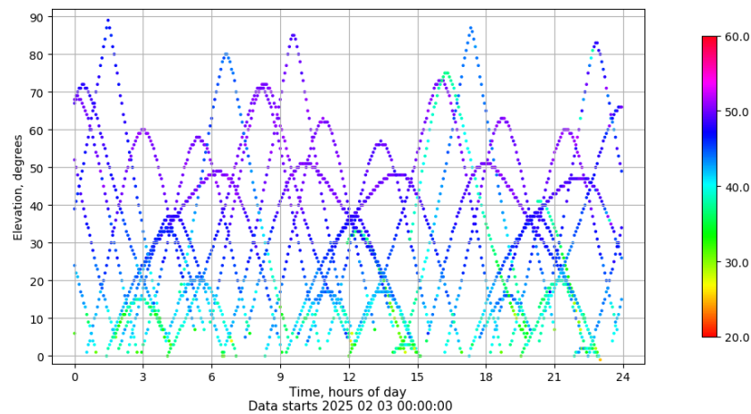
Time-elevation plot for station LP01. Signal to Noise S1C Data file LP0100ESP_R_2025034.xtr
