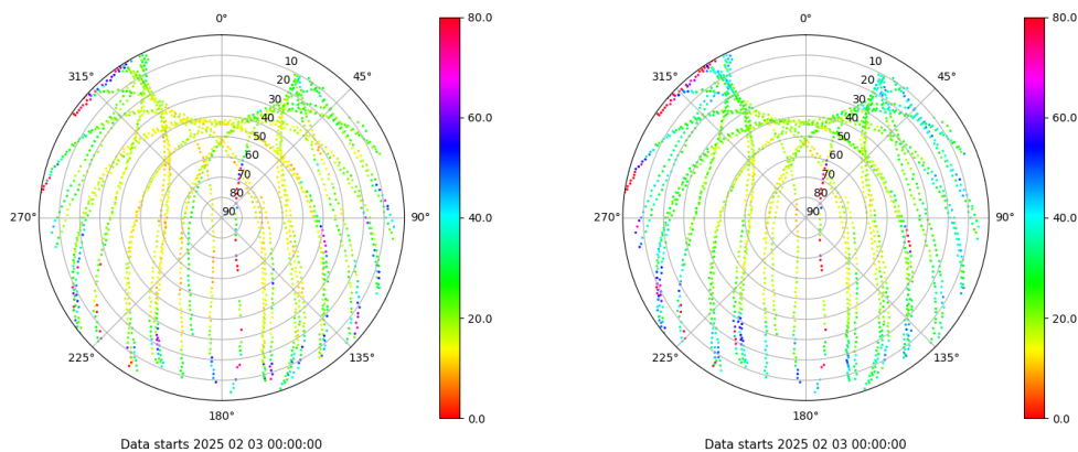
Skyplot for station LP01. Parameter M1C Data file LP0100ESP_R_2025034.xtr Skyplot for station LP01. Parameter M2C Data file LP0100ESP_R_2025034.xtr
