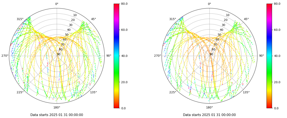
Skyplot for station LP01. Parameter M1C Data file LP0100ESP_R_2025031.xtr Skyplot for station LP01. Parameter M2X Data file LP0100ESP_R_2025031.xtr
