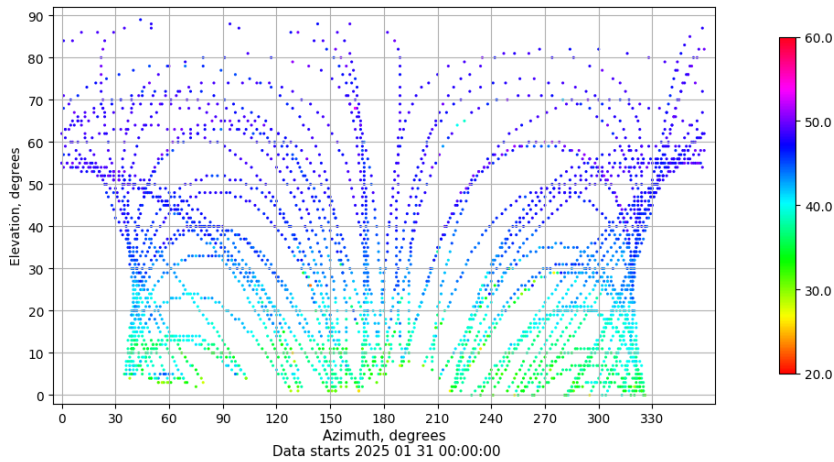
Azimuth-elevation plot for station LP01. Signal to Noise S1C Data file LP0100ESP_R_2025031.xtr
