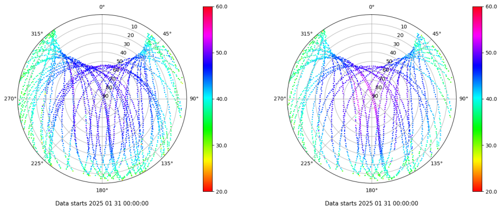
Skyplot for station LP01. Signal to Noise S1C Data file LP0100ESP_R_2025031.xtr Skyplot for station LP01. Signal to Noise S2X Data file LP0100ESP_R_2025031.xtr
