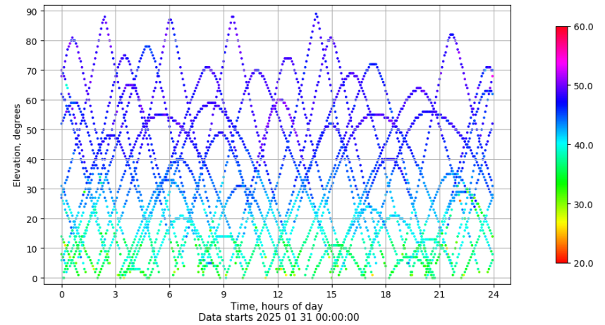
Time-elevation plot for station LP01. Signal to Noise S1C Data file LP0100ESP_R_2025031.xtr
