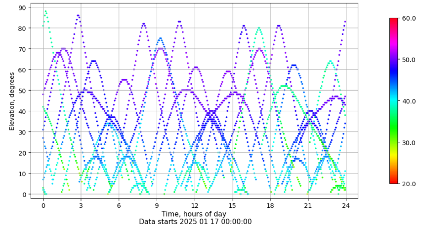
Time-elevation plot for station LP01. Signal to Noise S1C Data file LP0100ESP_R_2025017.xtr
