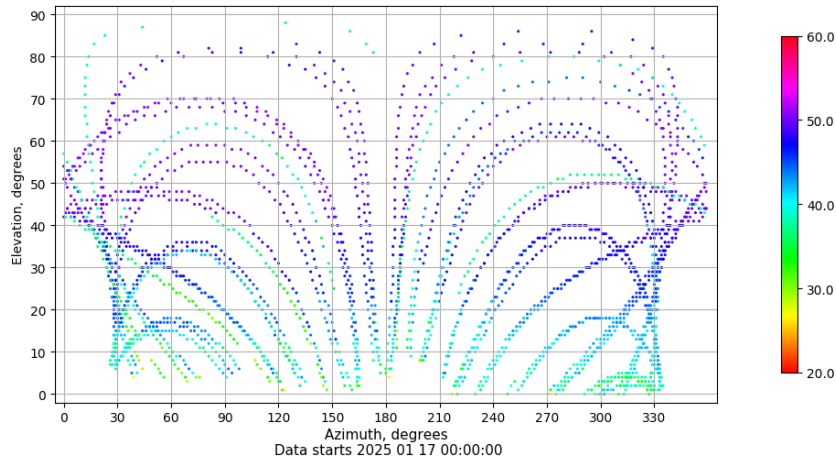
Azimuth-elevation plot for station LP01. Signal to Noise S1C Data file LP0100ESP_R_2025017.xtr
