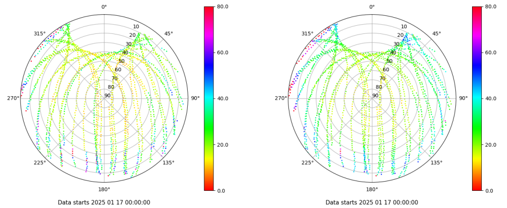
Skyplot for station LP01. Parameter M1C Data file LP0100ESP_R_2025017.xtr Skyplot for station LP01. Parameter M2C Data file LP0100ESP_R_2025017.xtr
