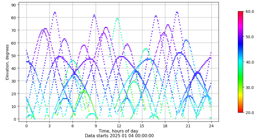
Time-elevation plot for station LP01. Signal to Noise S1C Data file LP0100ESP_R_2025004.xtr
