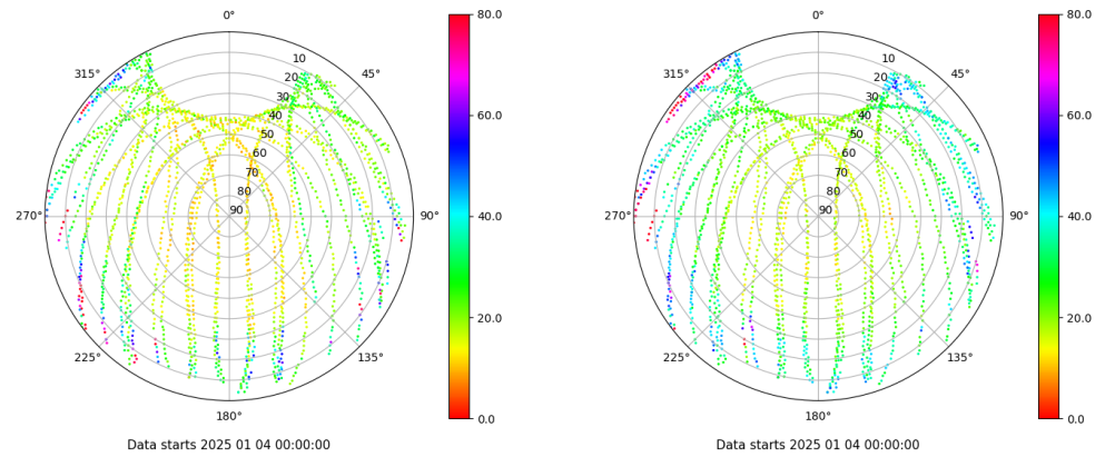
Skyplot for station LP01. Parameter M1C Data file LP0100ESP_R_2025004.xtr Skyplot for station LP01. Parameter M2C Data file LP0100ESP_R_2025004.xtr
