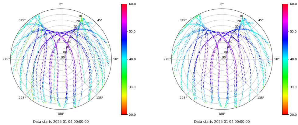
Skyplot for station LP01. Signal to Noise S1C Data file LP0100ESP_R_2025004.xtr Skyplot for station LP01. Signal to Noise S2C Data file LP0100ESP_R_2025004.xtr
