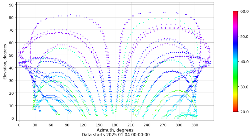
Azimuth-elevation plot for station LP01. Signal to Noise S1C Data file LP0100ESP_R_2025004.xtr
