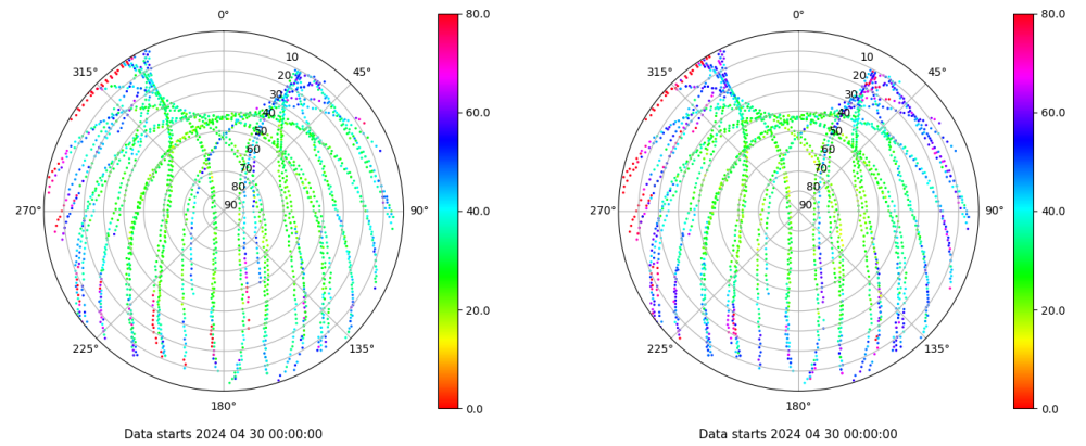
Skyplot for station LP01. Parameter M1C Data file LP0100ESP_R_2024121.xtr Skyplot for station LP01. Parameter M2C Data file LP0100ESP_R_2024121.xtr
