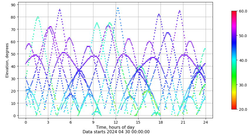
Time-elevation plot for station LP01. Signal to Noise S1C Data file LP0100ESP_R_2024121.xtr
