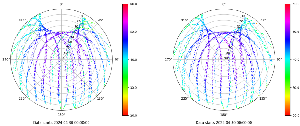
Skyplot for station LP01. Signal to Noise S1C Data file LP0100ESP_R_2024121.xtr Skyplot for station LP01. Signal to Noise S2C Data file LP0100ESP_R_2024121.xtr
