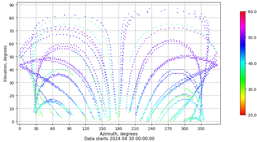
Azimuth-elevation plot for station LP01. Signal to Noise S1C Data file LP0100ESP_R_2024121.xtr
