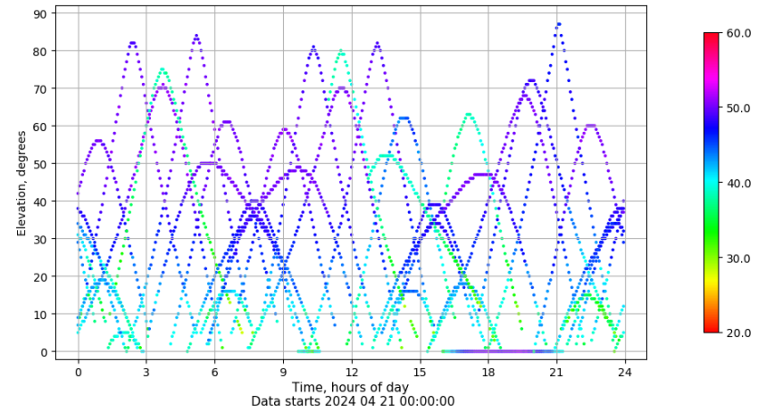
Time-elevation plot for station LP01. Signal to Noise S1C Data file LP0100ESP_R_2024112.xtr
