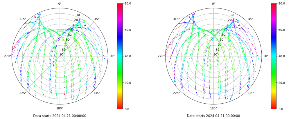
Skyplot for station LP01. Parameter M1C Data file LP0100ESP_R_2024112.xtr Skyplot for station LP01. Parameter M2C Data file LP0100ESP_R_2024112.xtr
