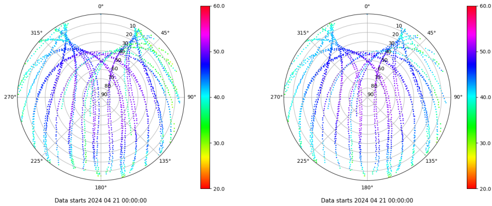
Skyplot for station LP01. Signal to Noise S1C Data file LP0100ESP_R_2024112.xtr Skyplot for station LP01. Signal to Noise S2C Data file LP0100ESP_R_2024112.xtr
