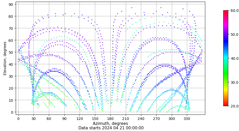
Azimuth-elevation plot for station LP01. Signal to Noise S1C Data file LP0100ESP_R_2024112.xtr
