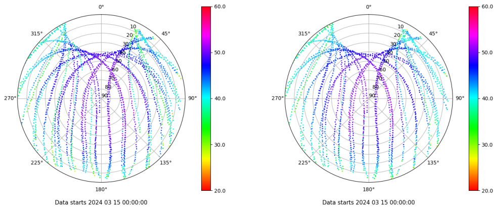
Skyplot for station LP01. Signal to Noise S1C Data file LP0100ESP_R_2024075.xtr Skyplot for station LP01. Signal to Noise S2C Data file LP0100ESP_R_2024075.xtr
