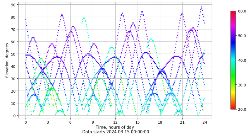
Time-elevation plot for station LP01. Signal to Noise S1C Data file LP0100ESP_R_2024075.xtr
