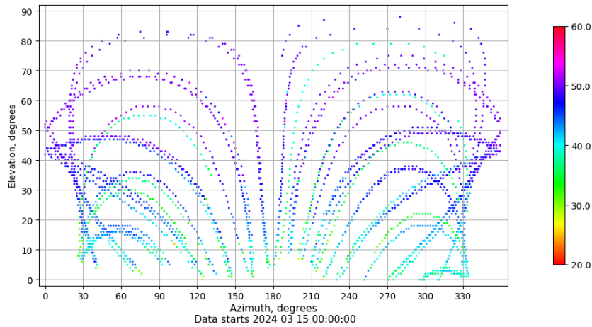
Azimuth-elevation plot for station LP01. Signal to Noise S1C Data file LP0100ESP_R_2024075.xtr
