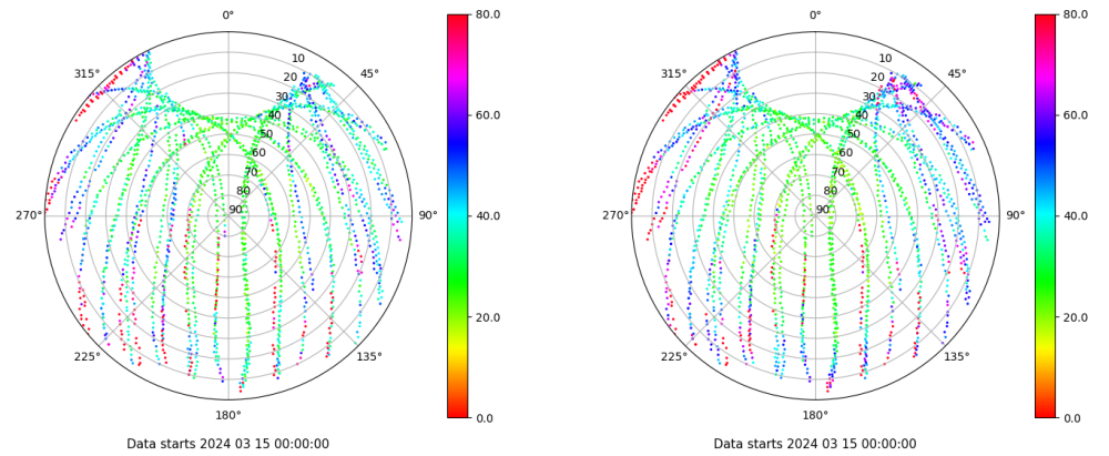
Skyplot for station LP01. Parameter M1C Data file LP0100ESP_R_2024075.xtr Skyplot for station LP01. Parameter M2C Data file LP0100ESP_R_2024075.xtr
