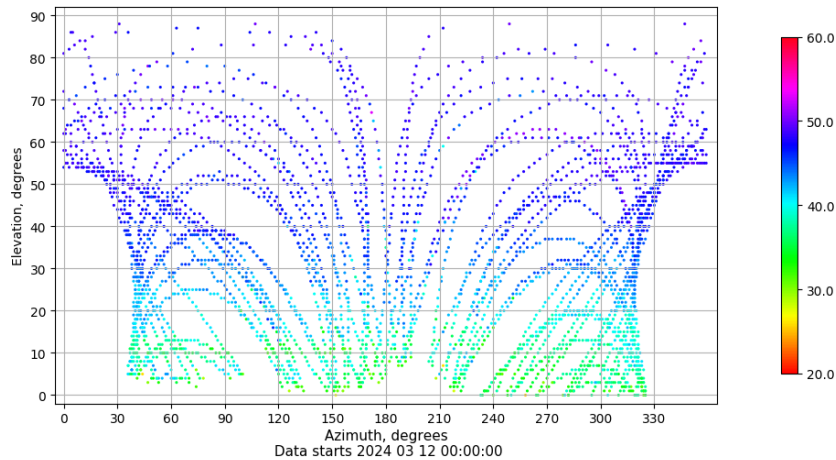
Azimuth-elevation plot for station LP01. Signal to Noise S1C Data file LP0100ESP_R_2024072.xtr
