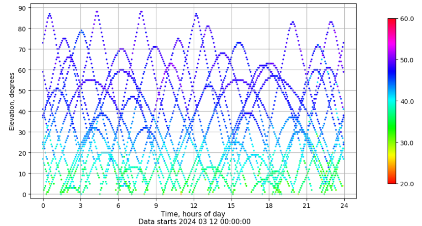
Time-elevation plot for station LP01. Signal to Noise S1C Data file LP0100ESP_R_2024072.xtr
