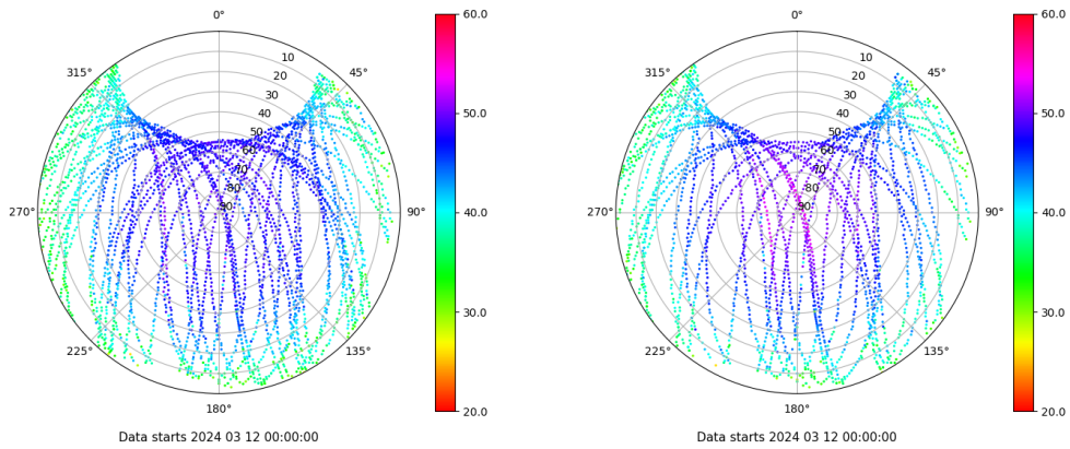
Skyplot for station LP01. Signal to Noise S1C Data file LP0100ESP_R_2024072.xtr Skyplot for station LP01. Signal to Noise S2X Data file LP0100ESP_R_2024072.xtr
