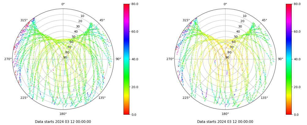
Skyplot for station LP01. Parameter M1C Data file LP0100ESP_R_2024072.xtr Skyplot for station LP01. Parameter M2X Data file LP0100ESP_R_2024072.xtr
