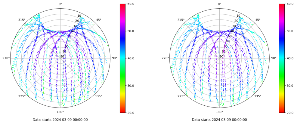
Skyplot for station LP01. Signal to Noise S1C Data file LP0100ESP_R_2024069.xtr Skyplot for station LP01. Signal to Noise S2C Data file LP0100ESP_R_2024069.xtr
