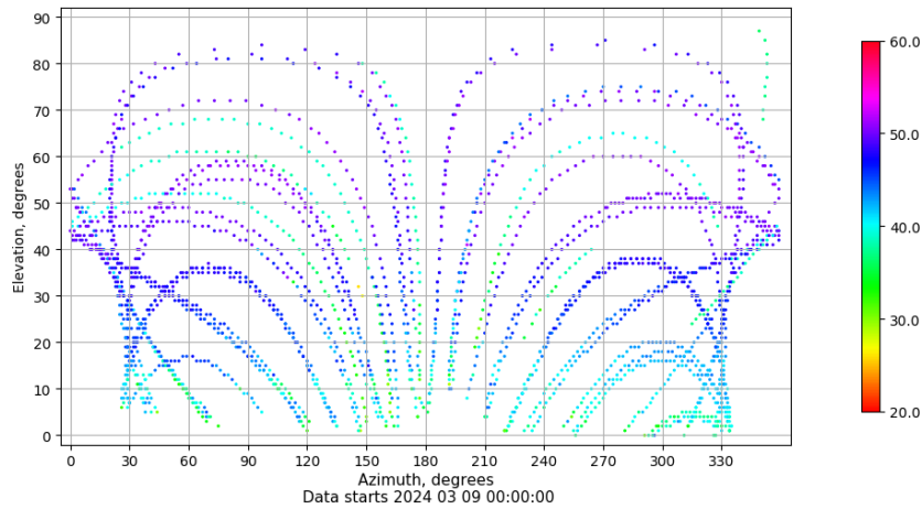
Azimuth-elevation plot for station LP01. Signal to Noise S1C Data file LP0100ESP_R_2024069.xtr
