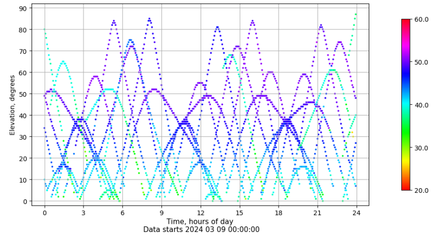
Time-elevation plot for station LP01. Signal to Noise S1C Data file LP0100ESP_R_2024069.xtr
