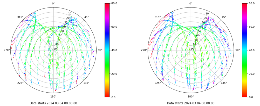
Skyplot for station LP01. Parameter M1C Data file LP0100ESP_R_2024064.xtr Skyplot for station LP01. Parameter M2C Data file LP0100ESP_R_2024064.xtr
