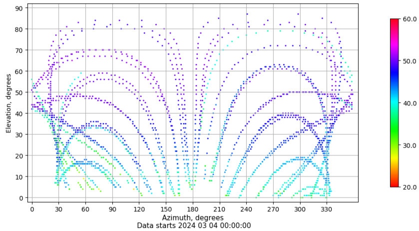
Azimuth-elevation plot for station LP01. Signal to Noise S1C Data file LP0100ESP_R_2024064.xtr
