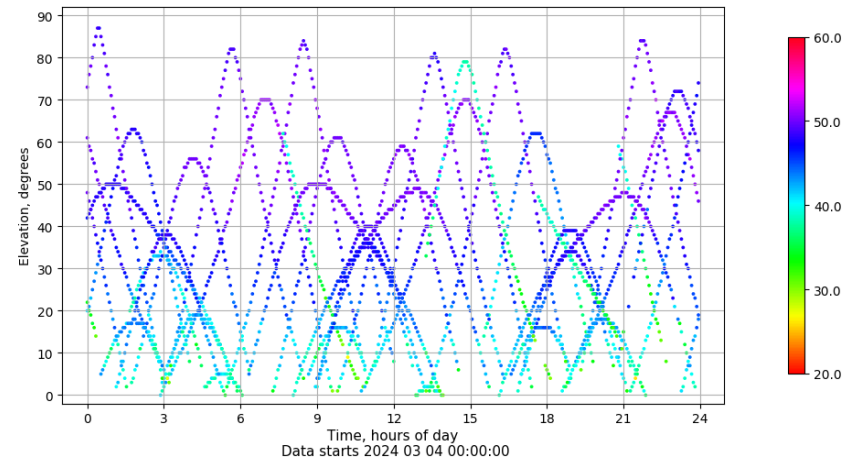
Time-elevation plot for station LP01. Signal to Noise S1C Data file LP0100ESP_R_2024064.xtr
