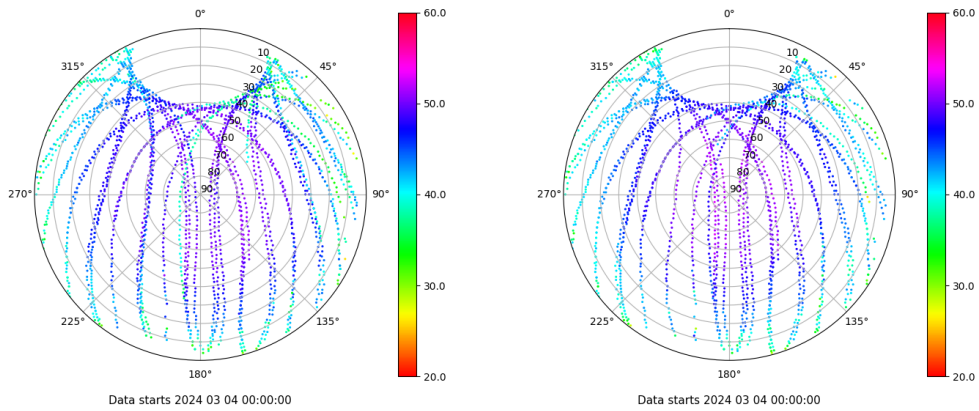
Skyplot for station LP01. Signal to Noise S1C Data file LP0100ESP_R_2024064.xtr Skyplot for station LP01. Signal to Noise S2C Data file LP0100ESP_R_2024064.xtr
