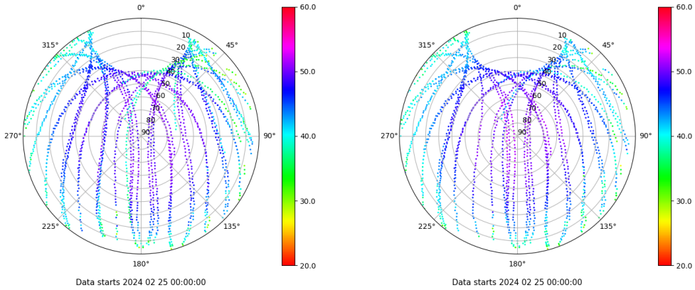
Skyplot for station LP01. Signal to Noise S1C Data file LP0100ESP_R_2024056.xtr Skyplot for station LP01. Signal to Noise S2C Data file LP0100ESP_R_2024056.xtr
