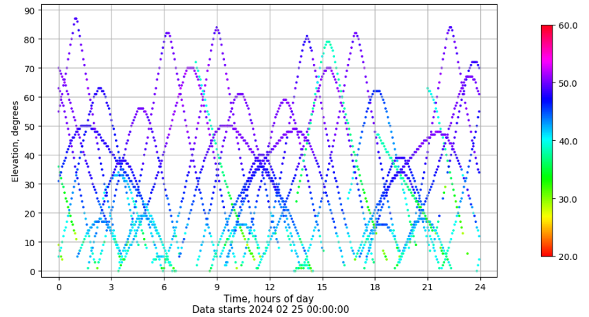
Time-elevation plot for station LP01. Signal to Noise S1C Data file LP0100ESP_R_2024056.xtr
