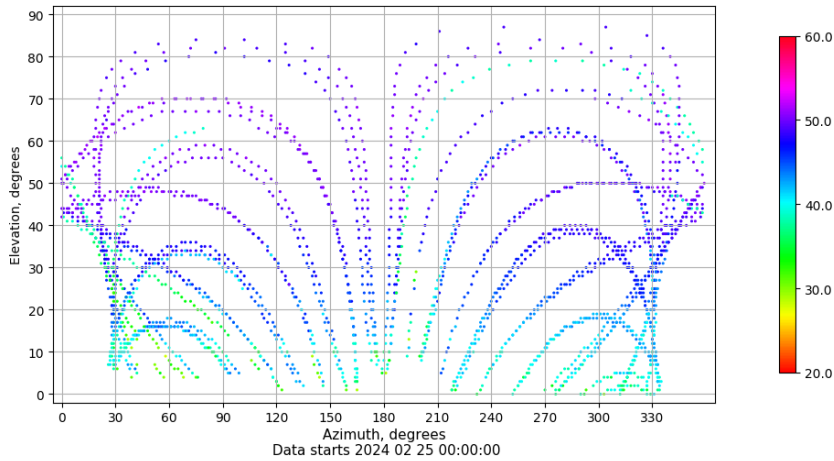
Azimuth-elevation plot for station LP01. Signal to Noise S1C Data file LP0100ESP_R_2024056.xtr
