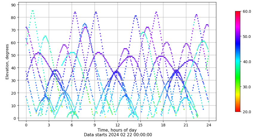
Time-elevation plot for station LP01. Signal to Noise S1C Data file LP0100ESP_R_2024053.xtr
