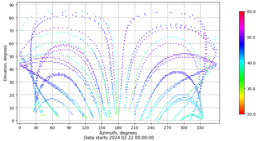
Azimuth-elevation plot for station LP01. Signal to Noise S1C Data file LP0100ESP_R_2024053.xtr
