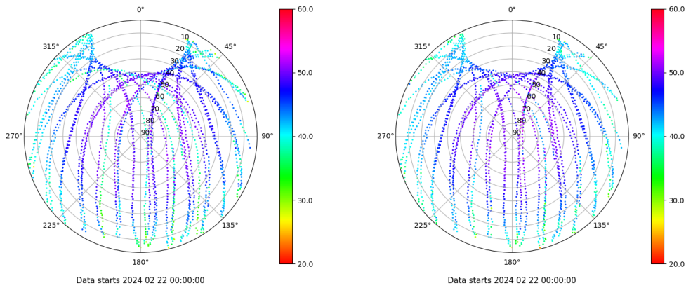
Skyplot for station LP01. Signal to Noise S1C Data file LP0100ESP_R_2024053.xtr Skyplot for station LP01. Signal to Noise S2C Data file LP0100ESP_R_2024053.xtr
