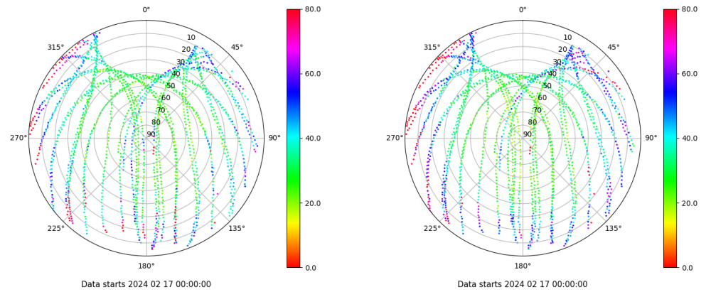
Skyplot for station LP01. Parameter M1C Data file LP0100ESP_R_2024048.xtr Skyplot for station LP01. Parameter M2C Data file LP0100ESP_R_2024048.xtr
