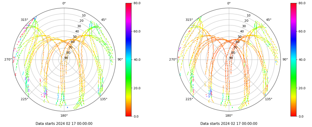
Skyplot for station LP01. Parameter M1X Data file LP0100ESP_R_2024048.xtr Skyplot for station LP01. Parameter M5X Data file LP0100ESP_R_2024048.xtr
