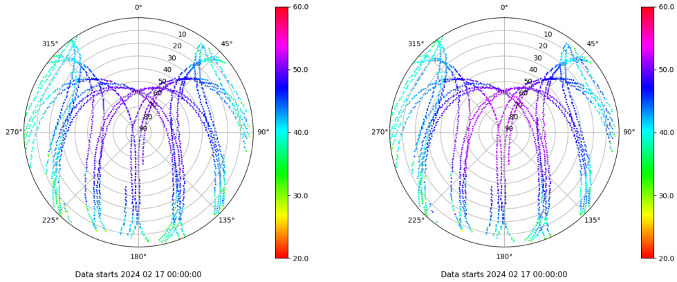
Skyplot for station LP01. Signal to Noise S1X Data file LP0100ESP_R_2024048.xtr Skyplot for station LP01. Signal to Noise S5X Data file LP0100ESP_R_2024048.xtr
