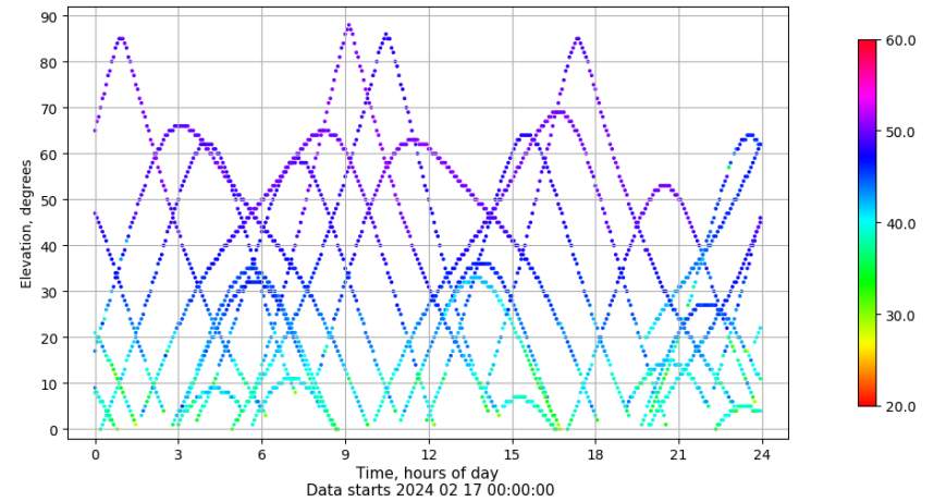
Time-elevation plot for station LP01. Signal to Noise S1X Data file LP0100ESP_R_2024048.xtr
