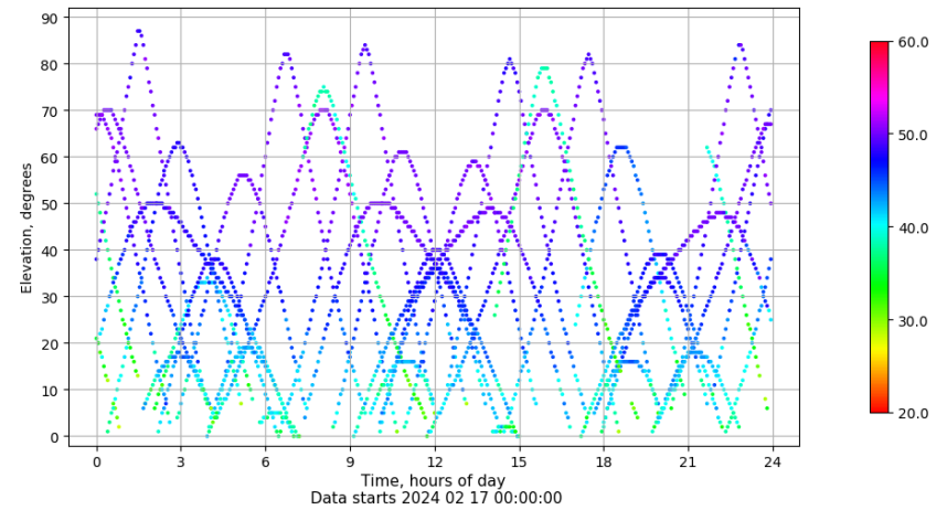
Time-elevation plot for station LP01. Signal to Noise S1C Data file LP0100ESP_R_2024048.xtr
