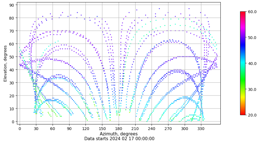
Azimuth-elevation plot for station LP01. Signal to Noise S1C Data file LP0100ESP_R_2024048.xtr
