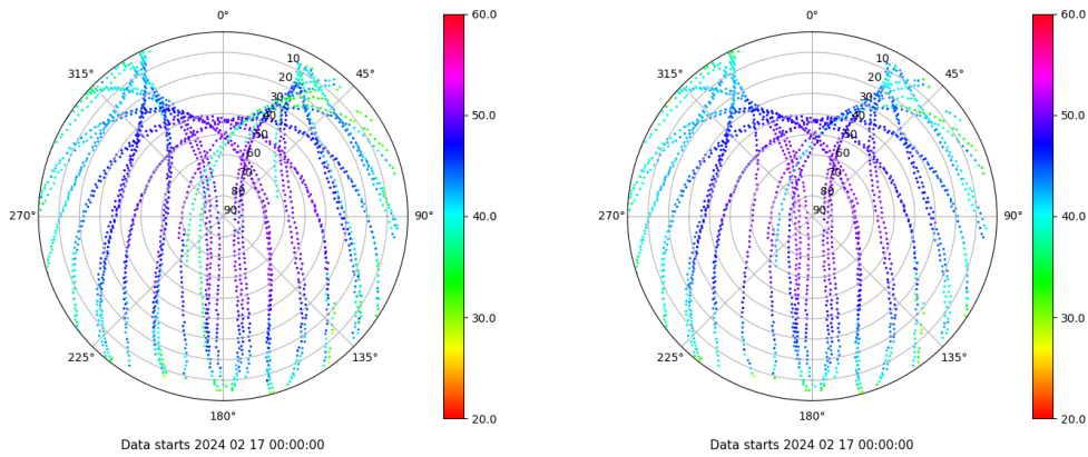
Skyplot for station LP01. Signal to Noise S1C Data file LP0100ESP_R_2024048.xtr Skyplot for station LP01. Signal to Noise S2C Data file LP0100ESP_R_2024048.xtr
