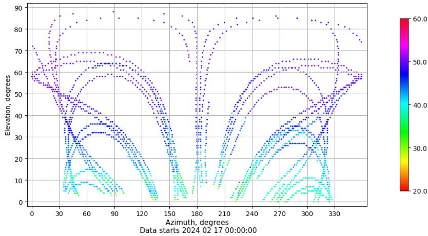
Azimuth-elevation plot for station LP01. Signal to Noise S1X Data file LP0100ESP_R_2024048.xtr
