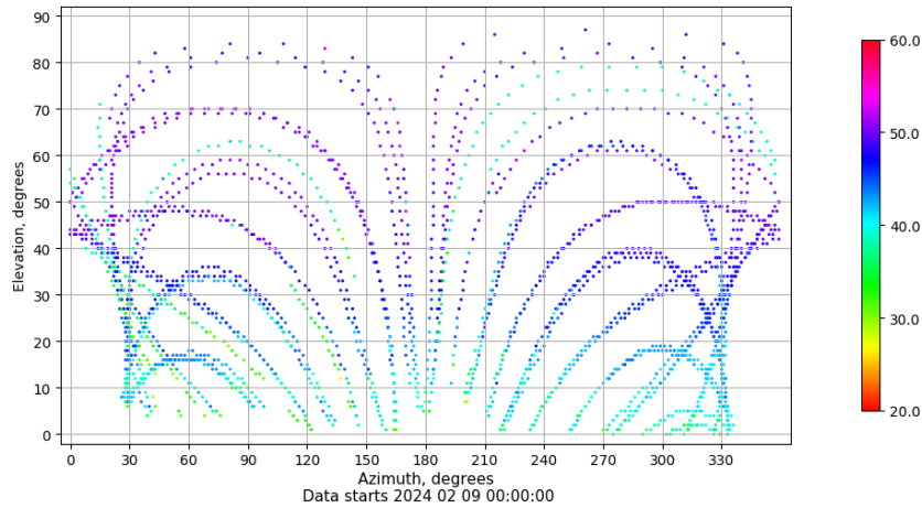
Azimuth-elevation plot for station LP01. Signal to Noise S1C Data file LP0100ESP_R_2024040.xtr
