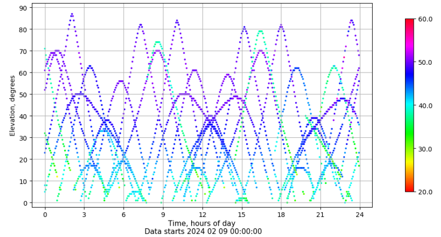
Time-elevation plot for station LP01. Signal to Noise S1C Data file LP0100ESP_R_2024040.xtr
