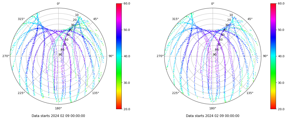
Skyplot for station LP01. Signal to Noise S1C Data file LP0100ESP_R_2024040.xtr Skyplot for station LP01. Signal to Noise S2C Data file LP0100ESP_R_2024040.xtr
