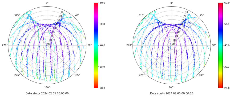
Skyplot for station LP01. Signal to Noise S1C Data file LP0100ESP_R_2024036.xtr Skyplot for station LP01. Signal to Noise S2C Data file LP0100ESP_R_2024036.xtr
