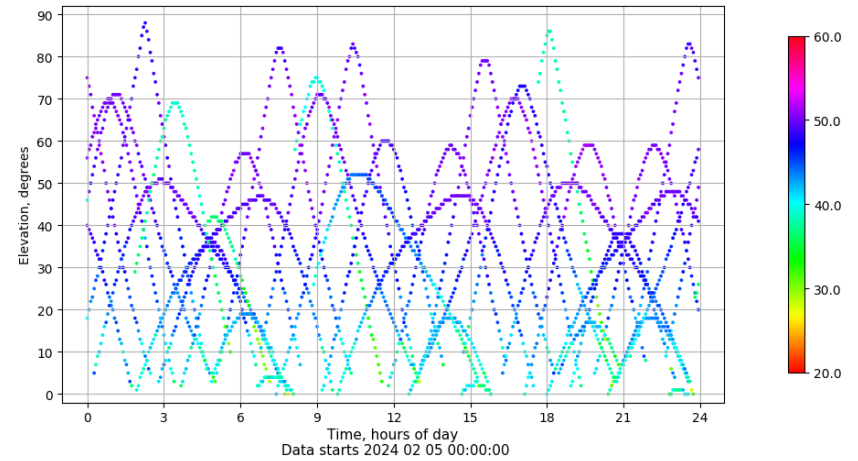
Time-elevation plot for station LP01. Signal to Noise S1C Data file LP0100ESP_R_2024036.xtr
