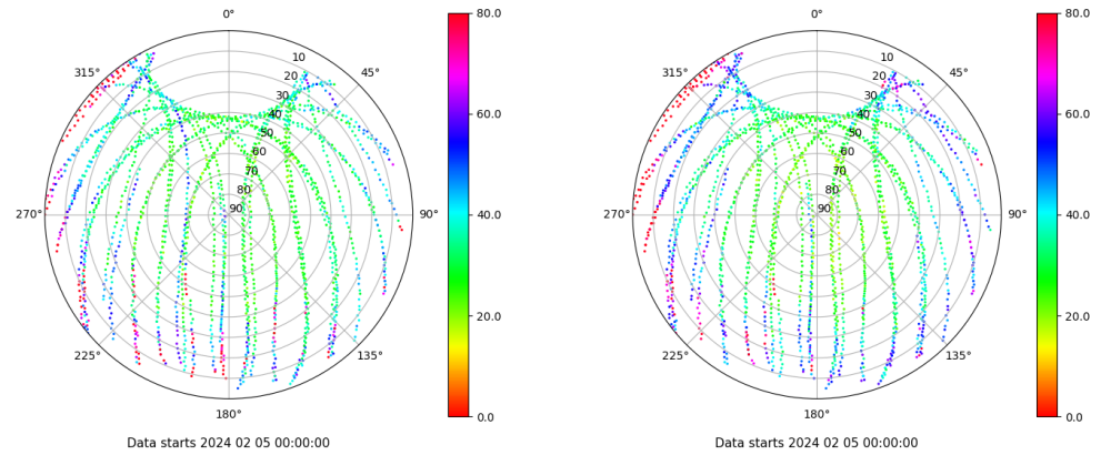
Skyplot for station LP01. Parameter M1C Data file LP0100ESP_R_2024036.xtr Skyplot for station LP01. Parameter M2C Data file LP0100ESP_R_2024036.xtr
