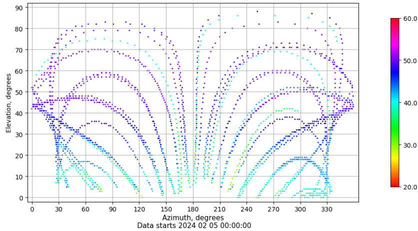
Azimuth-elevation plot for station LP01. Signal to Noise S1C Data file LP0100ESP_R_2024036.xtr
