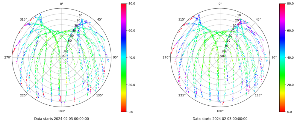
Skyplot for station LP01. Parameter M1C Data file LP0100ESP_R_2024034.xtr Skyplot for station LP01. Parameter M2C Data file LP0100ESP_R_2024034.xtr
