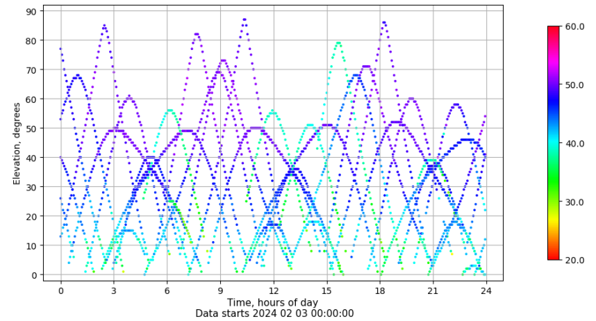
Time-elevation plot for station LP01. Signal to Noise S1C Data file LP0100ESP_R_2024034.xtr
