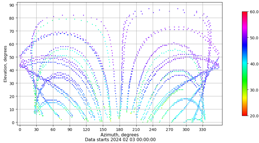
Azimuth-elevation plot for station LP01. Signal to Noise S1C Data file LP0100ESP_R_2024034.xtr
