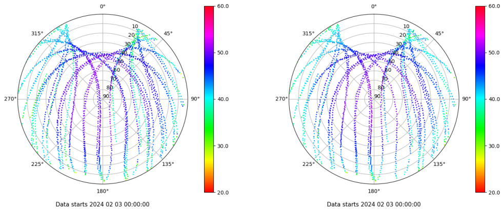
Skyplot for station LP01. Signal to Noise S1C Data file LP0100ESP_R_2024034.xtr Skyplot for station LP01. Signal to Noise S2C Data file LP0100ESP_R_2024034.xtr
