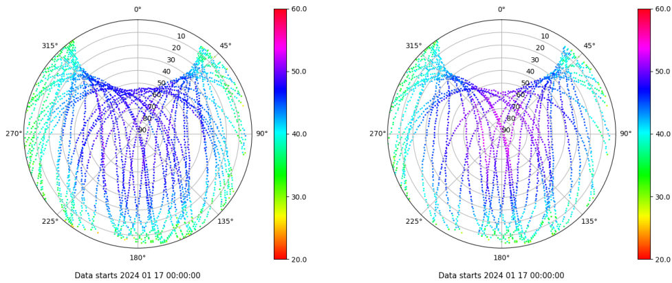
Skyplot for station LP01. Signal to Noise S1C Data file LP0100ESP_R_2024017.xtr Skyplot for station LP01. Signal to Noise S2X Data file LP0100ESP_R_2024017.xtr
