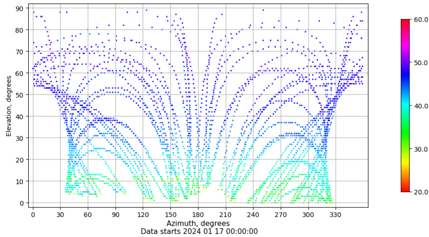
Azimuth-elevation plot for station LP01. Signal to Noise S1C Data file LP0100ESP_R_2024017.xtr
