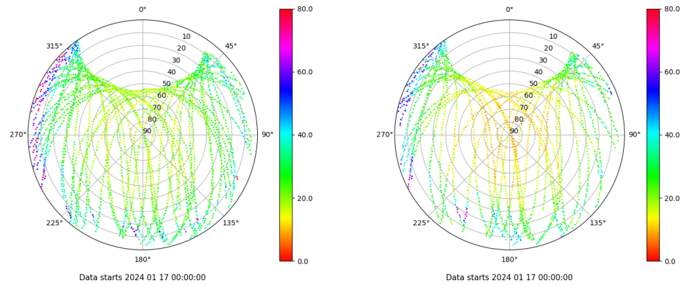
Skyplot for station LP01. Parameter M1C Data file LP0100ESP_R_2024017.xtr Skyplot for station LP01. Parameter M2X Data file LP0100ESP_R_2024017.xtr
