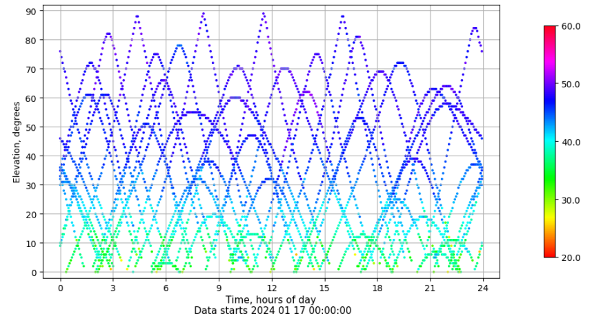
Time-elevation plot for station LP01. Signal to Noise S1C Data file LP0100ESP_R_2024017.xtr
