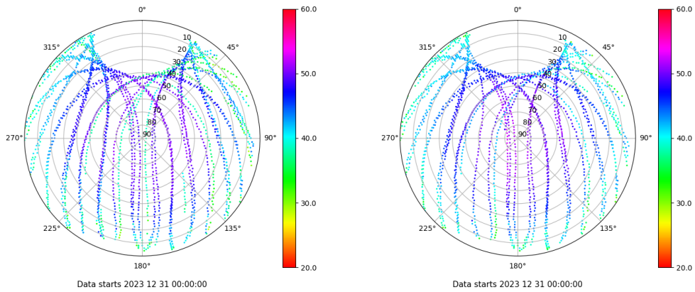
Skyplot for station LP01. Signal to Noise S1C Data file LP0100ESP_R_2023365.xtr Skyplot for station LP01. Signal to Noise S2C Data file LP0100ESP_R_2023365.xtr
