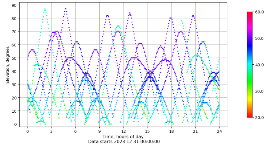
Time-elevation plot for station LP01. Signal to Noise S1C Data file LP0100ESP_R_2023365.xtr
