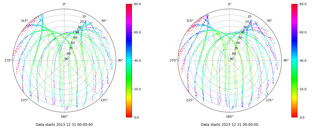
Skyplot for station LP01. Parameter M1C Data file LP0100ESP_R_2023365.xtr Skyplot for station LP01. Parameter M2C Data file LP0100ESP_R_2023365.xtr
