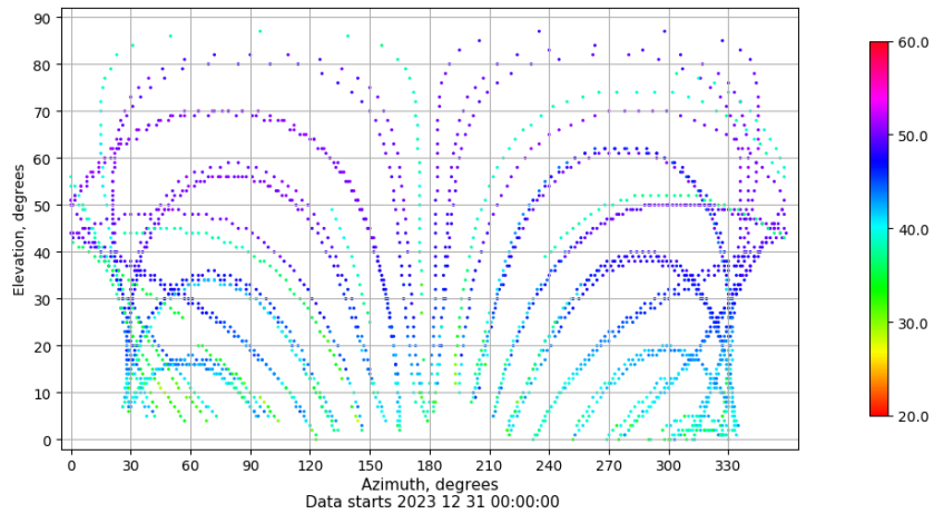
Azimuth-elevation plot for station LP01. Signal to Noise S1C Data file LP0100ESP_R_2023365.xtr
