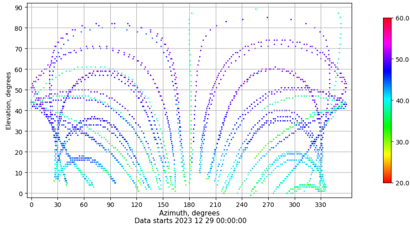
Azimuth-elevation plot for station LP01. Signal to Noise S1C Data file LP0100ESP_R_2023363.xtr
