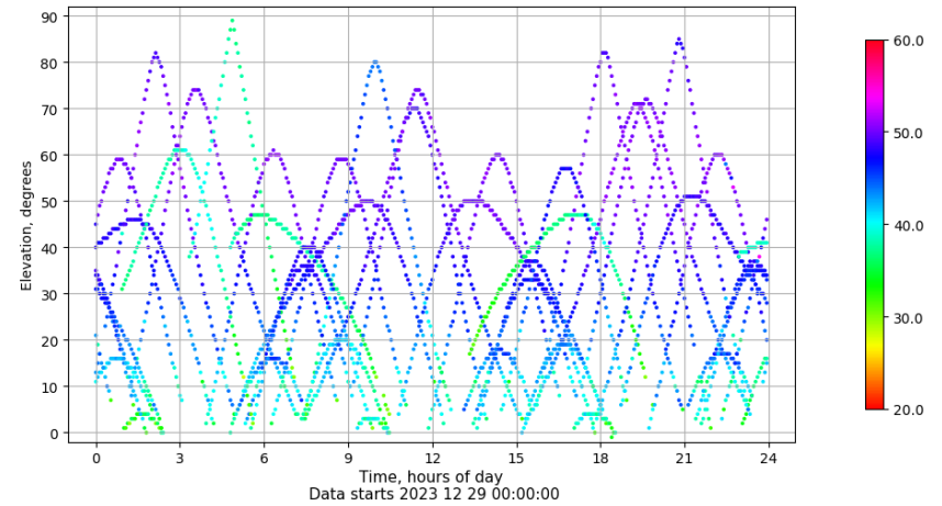
Time-elevation plot for station LP01. Signal to Noise S1C Data file LP0100ESP_R_2023363.xtr
