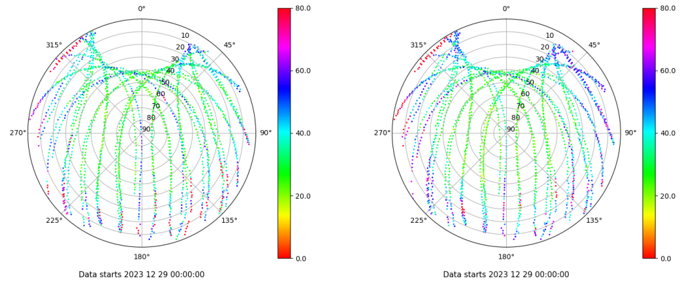
Skyplot for station LP01. Parameter M1C Data file LP0100ESP_R_2023363.xtr Skyplot for station LP01. Parameter M2C Data file LP0100ESP_R_2023363.xtr
