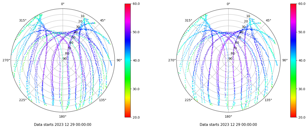
Skyplot for station LP01. Signal to Noise S1C Data file LP0100ESP_R_2023363.xtr Skyplot for station LP01. Signal to Noise S2C Data file LP0100ESP_R_2023363.xtr
