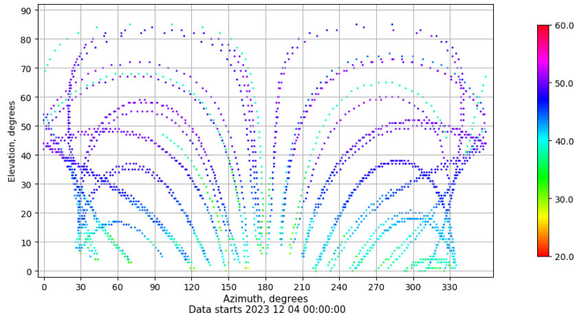
Azimuth-elevation plot for station LP01. Signal to Noise S1C Data file LP0100ESP_R_2023338.xtr
