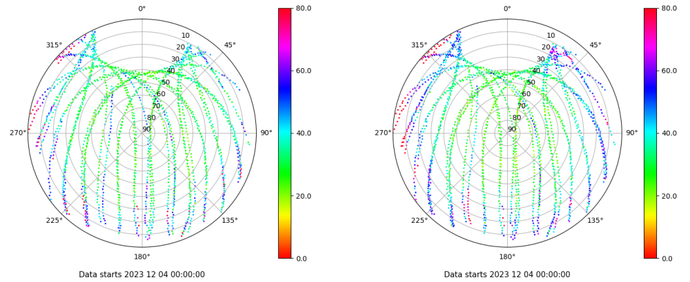
Skyplot for station LP01. Parameter M1C Data file LP0100ESP_R_2023338.xtr Skyplot for station LP01. Parameter M2C Data file LP0100ESP_R_2023338.xtr
