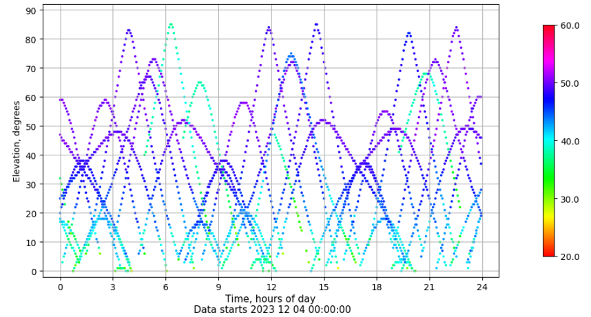
Time-elevation plot for station LP01. Signal to Noise S1C Data file LP0100ESP_R_2023338.xtr
