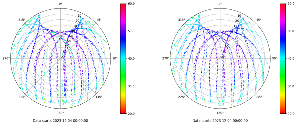
Skyplot for station LP01. Signal to Noise S1C Data file LP0100ESP_R_2023338.xtr Skyplot for station LP01. Signal to Noise S2C Data file LP0100ESP_R_2023338.xtr
