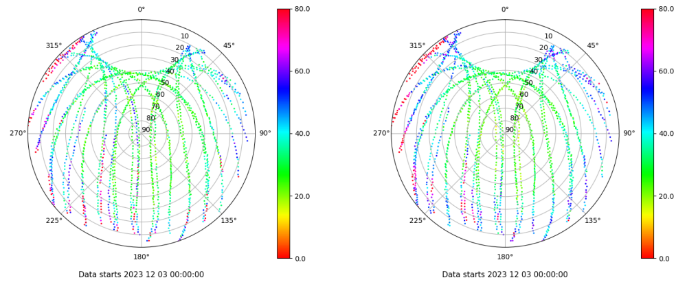
Skyplot for station LP01. Parameter M1C Data file LP0100ESP_R_2023337.xtr Skyplot for station LP01. Parameter M2C Data file LP0100ESP_R_2023337.xtr
