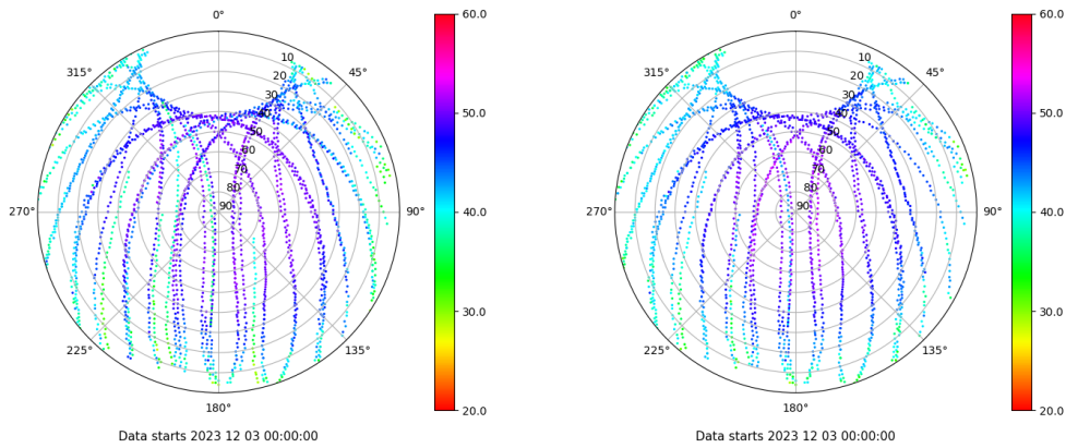
Skyplot for station LP01. Signal to Noise S1C Data file LP0100ESP_R_2023337.xtr Skyplot for station LP01. Signal to Noise S2C Data file LP0100ESP_R_2023337.xtr
