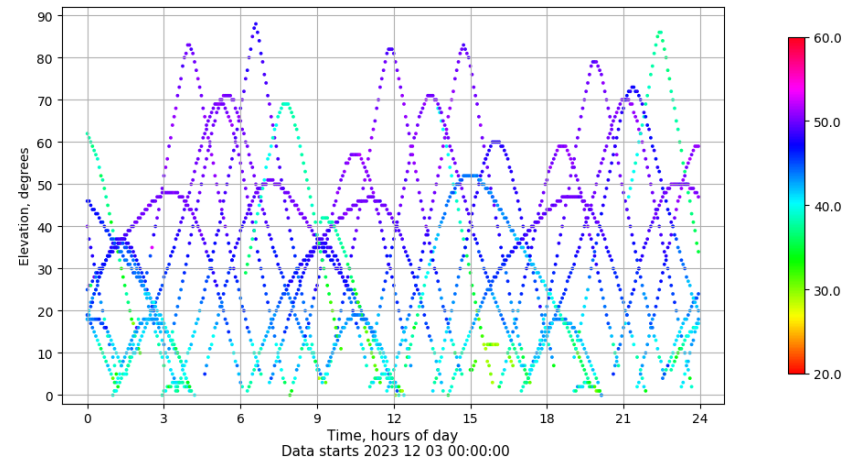
Time-elevation plot for station LP01. Signal to Noise S1C Data file LP0100ESP_R_2023337.xtr
