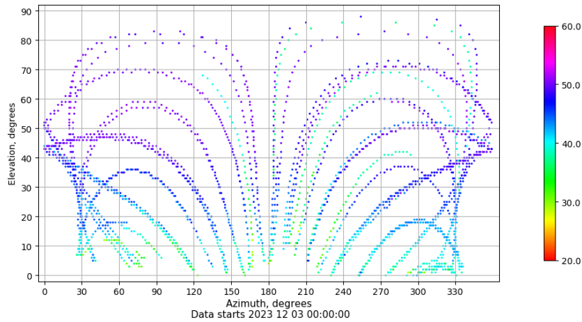
Azimuth-elevation plot for station LP01. Signal to Noise S1C Data file LP0100ESP_R_2023337.xtr
