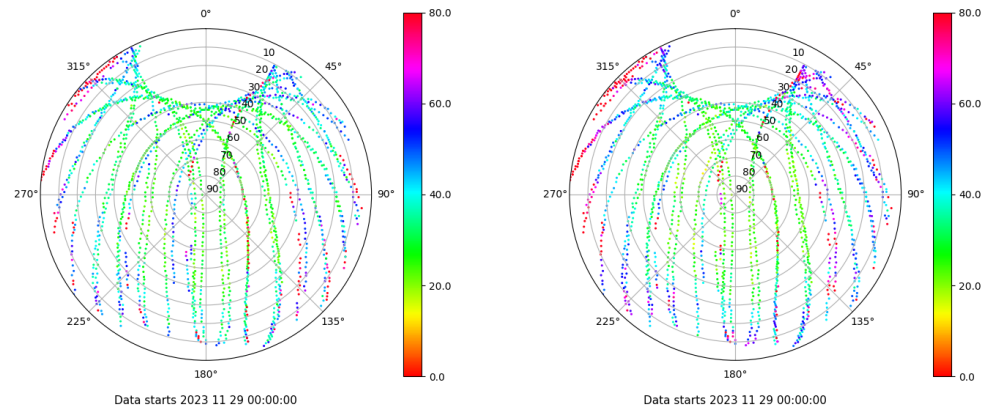
Skyplot for station LP01. Parameter M1C Data file LP0100ESP_R_2023333.xtr Skyplot for station LP01. Parameter M2C Data file LP0100ESP_R_2023333.xtr
