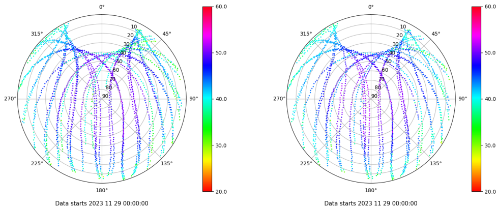
Skyplot for station LP01. Signal to Noise S1C Data file LP0100ESP_R_2023333.xtr Skyplot for station LP01. Signal to Noise S2C Data file LP0100ESP_R_2023333.xtr
