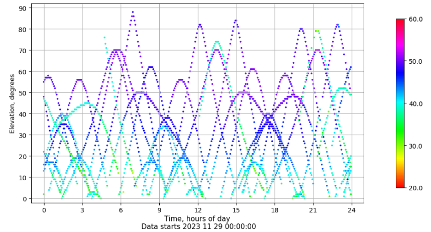
Time-elevation plot for station LP01. Signal to Noise S1C Data file LP0100ESP_R_2023333.xtr
