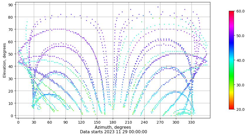
Azimuth-elevation plot for station LP01. Signal to Noise S1C Data file LP0100ESP_R_2023333.xtr
