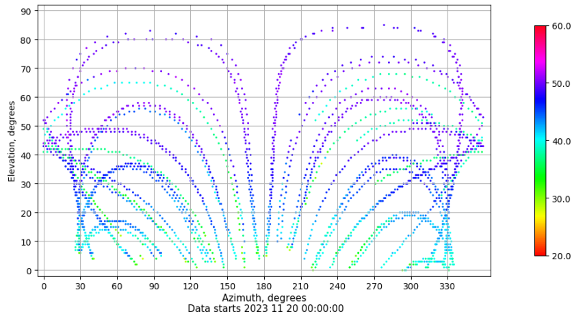
Azimuth-elevation plot for station LP01. Signal to Noise S1C Data file LP0100ESP_R_2023324.xtr
