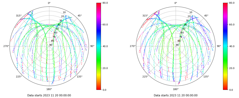
Skyplot for station LP01. Parameter M1C Data file LP0100ESP_R_2023324.xtr Skyplot for station LP01. Parameter M2C Data file LP0100ESP_R_2023324.xtr
