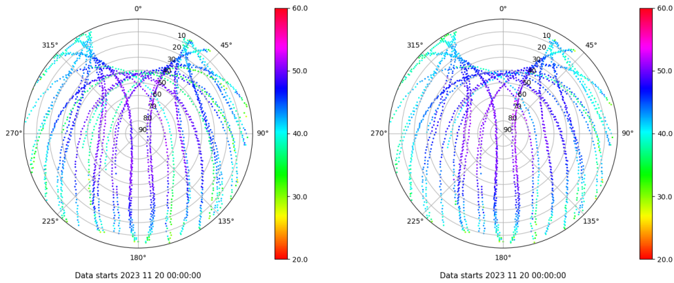
Skyplot for station LP01. Signal to Noise S1C Data file LP0100ESP_R_2023324.xtr Skyplot for station LP01. Signal to Noise S2C Data file LP0100ESP_R_2023324.xtr
