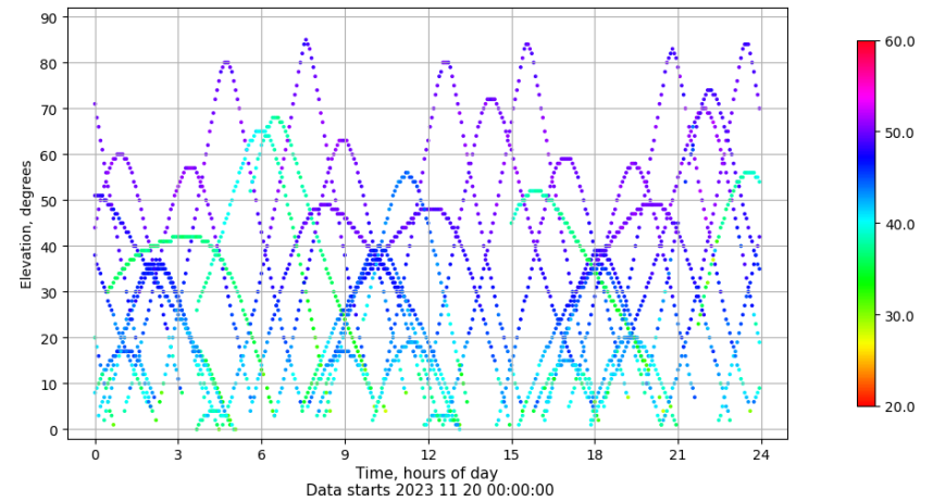
Time-elevation plot for station LP01. Signal to Noise S1C Data file LP0100ESP_R_2023324.xtr
