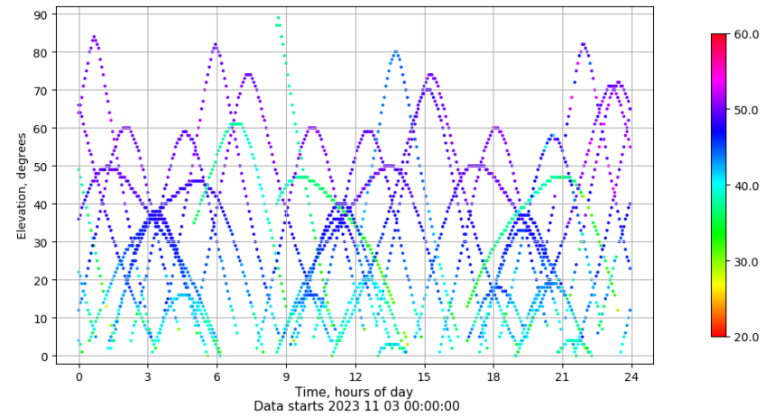
Time-elevation plot for station LP01. Signal to Noise S1C Data file LP0100ESP_R_2023307.xtr
