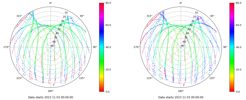
Skyplot for station LP01. Parameter M1C Data file LP0100ESP_R_2023307.xtr Skyplot for station LP01. Parameter M2C Data file LP0100ESP_R_2023307.xtr
