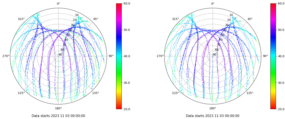
Skyplot for station LP01. Signal to Noise S1C Data file LP0100ESP_R_2023307.xtr Skyplot for station LP01. Signal to Noise S2C Data file LP0100ESP_R_2023307.xtr
