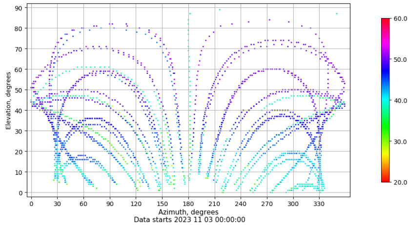
Azimuth-elevation plot for station LP01. Signal to Noise S1C Data file LP0100ESP_R_2023307.xtr
